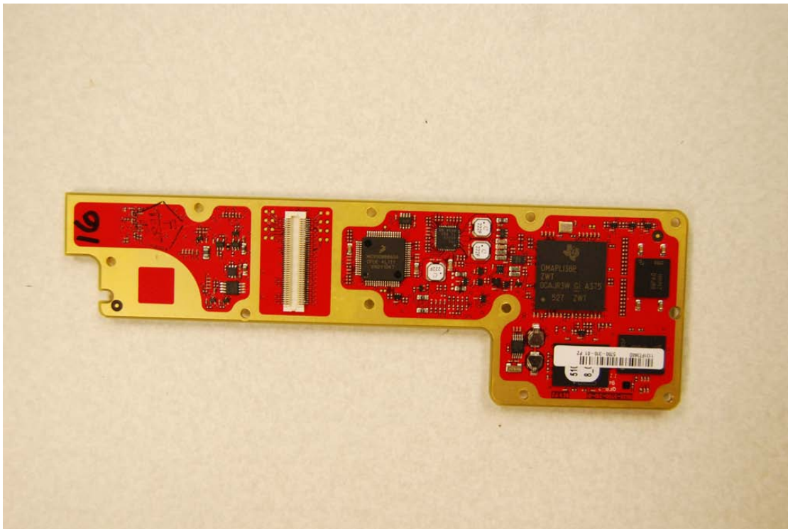
Audio/Logic PC Board Front
