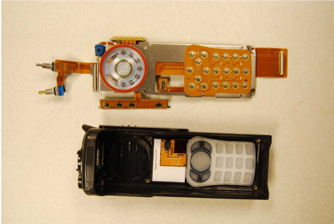
Radio Front with Display Modules Installed and Main Flex Assembly
