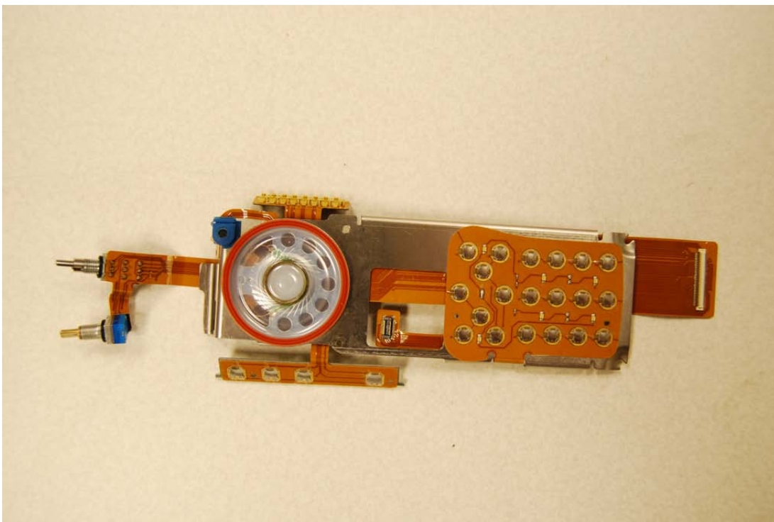
Main Flex PC Board Front
