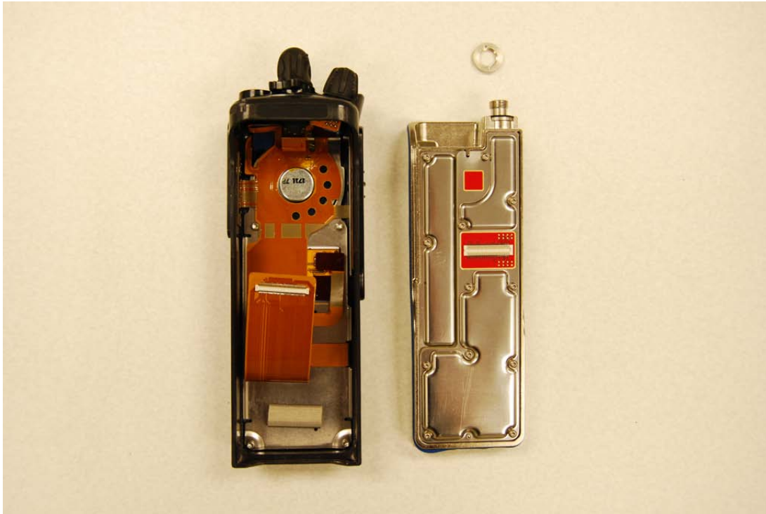
Radio Assembly Opened
