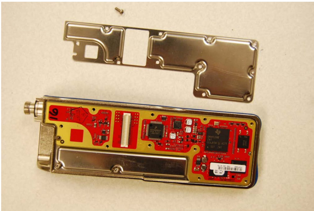
Radio Chassis Assembly with Shield Removed Showing Audio/Logic PC Board
