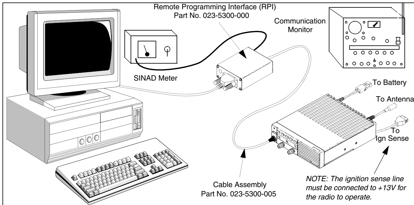
Figure 6-1 Alignment Setup
