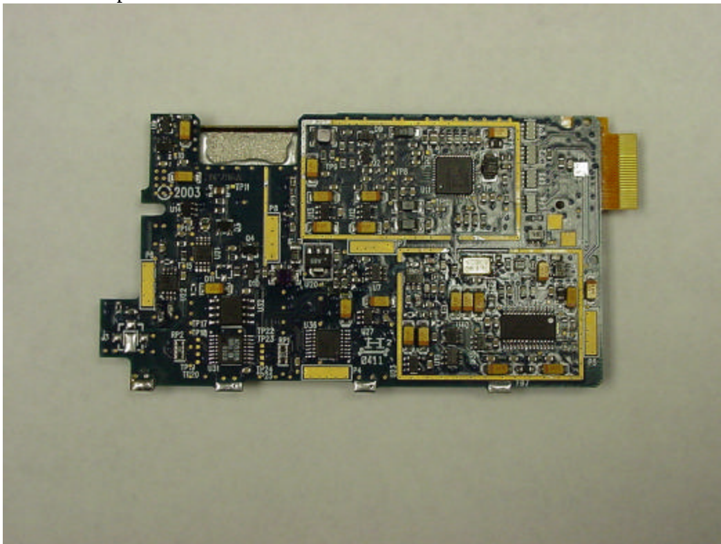
RF module bottom with shields removed
