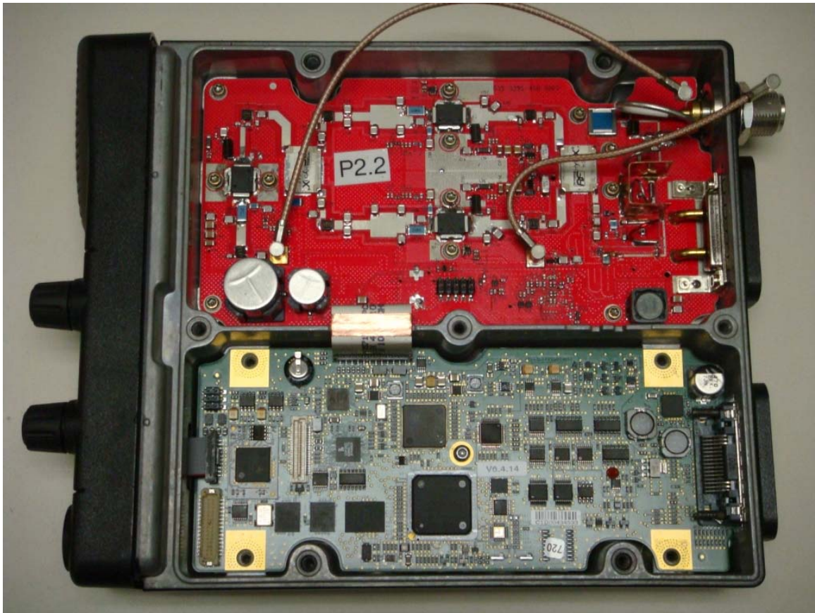
Radio with cover removed and RF assembly removed
