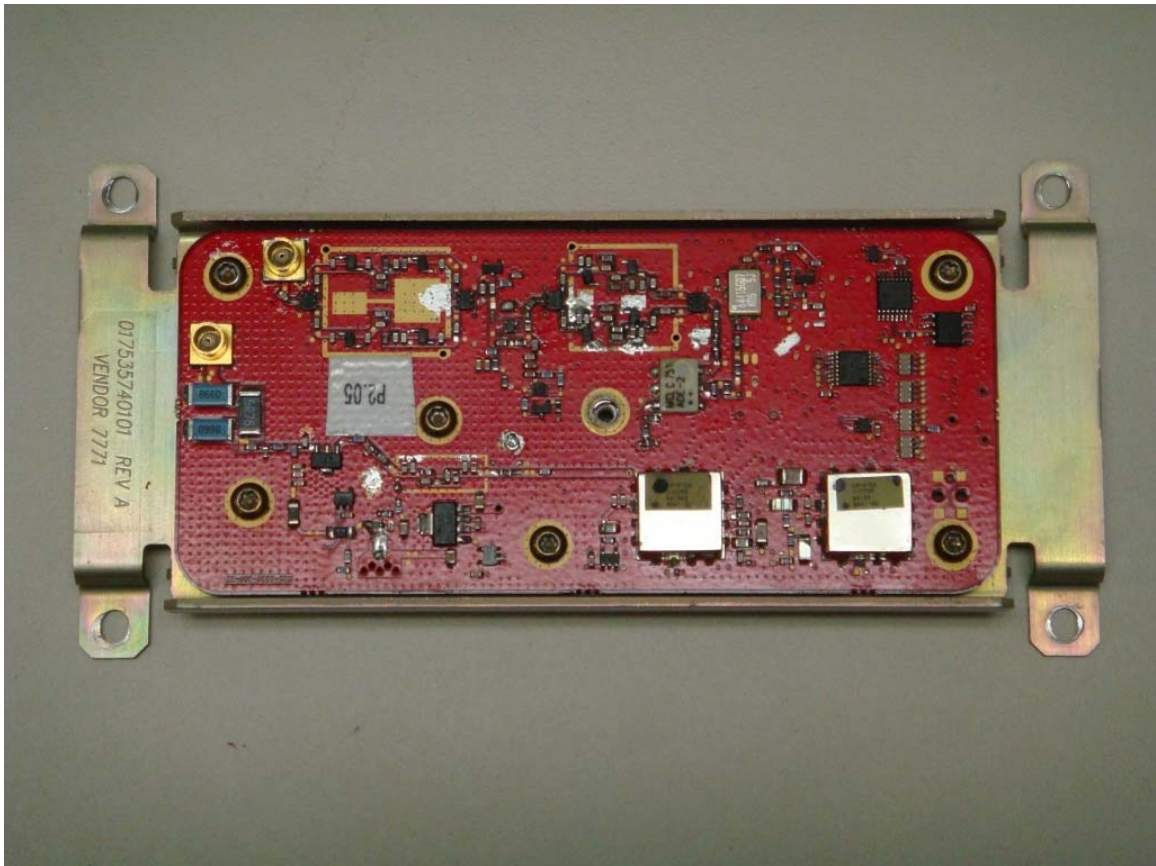
RF board front in carrier with shield removed
