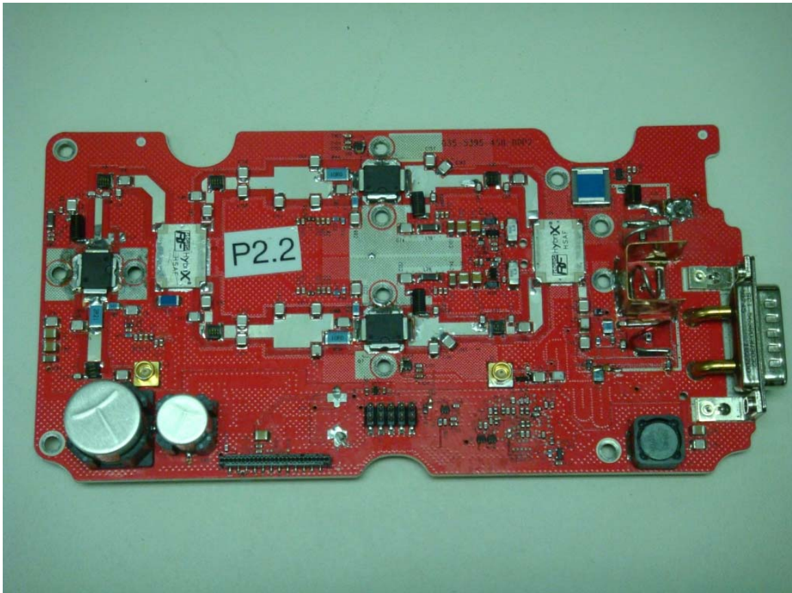
PA board front
