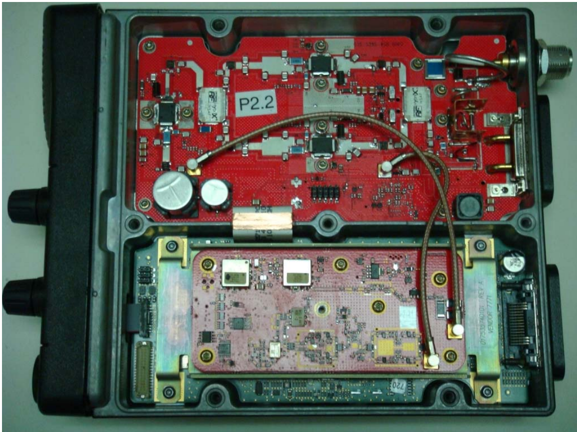
Radio with cover removed and RF Shield removed
