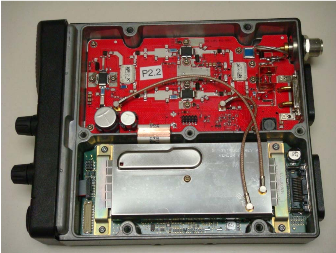
Radio bottom with cover removed
