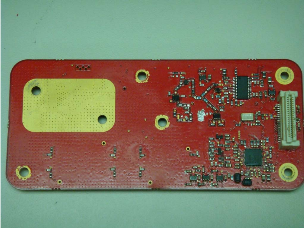
RF board rear
