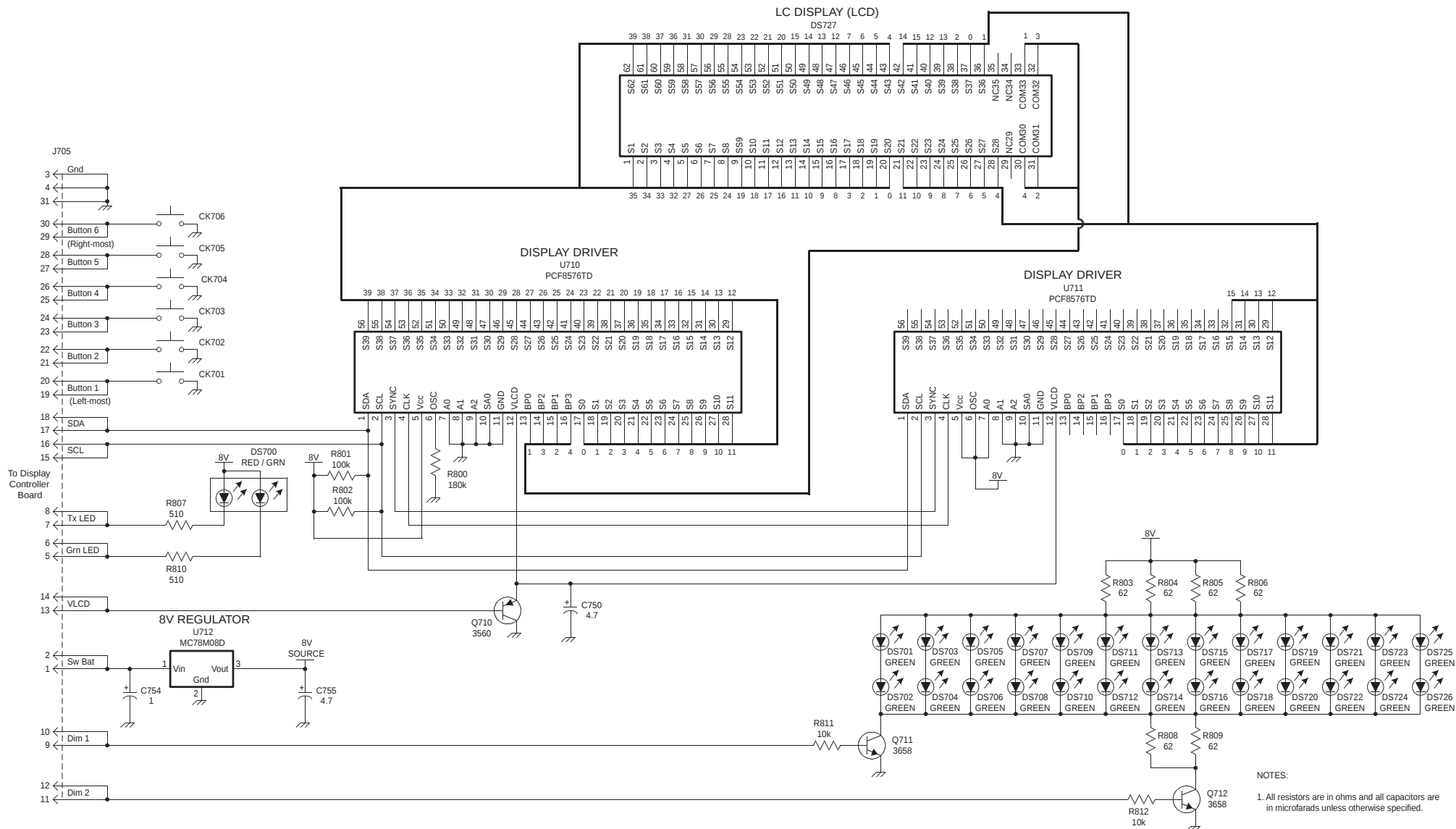
DISPLAY BOARD SCHEMATIC
