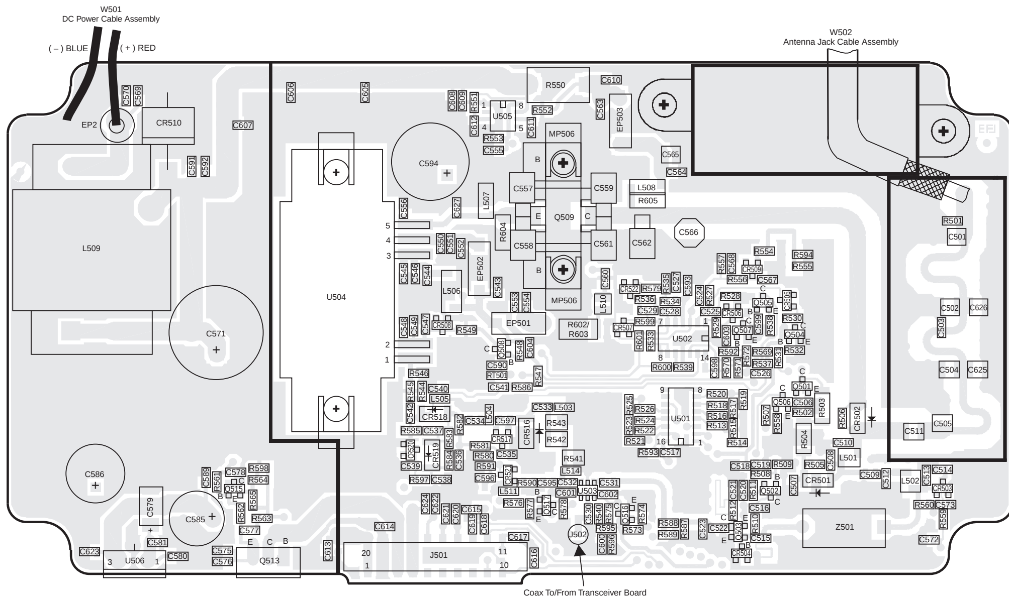
800 MHZ 50W PA BOARD LAYOUT
