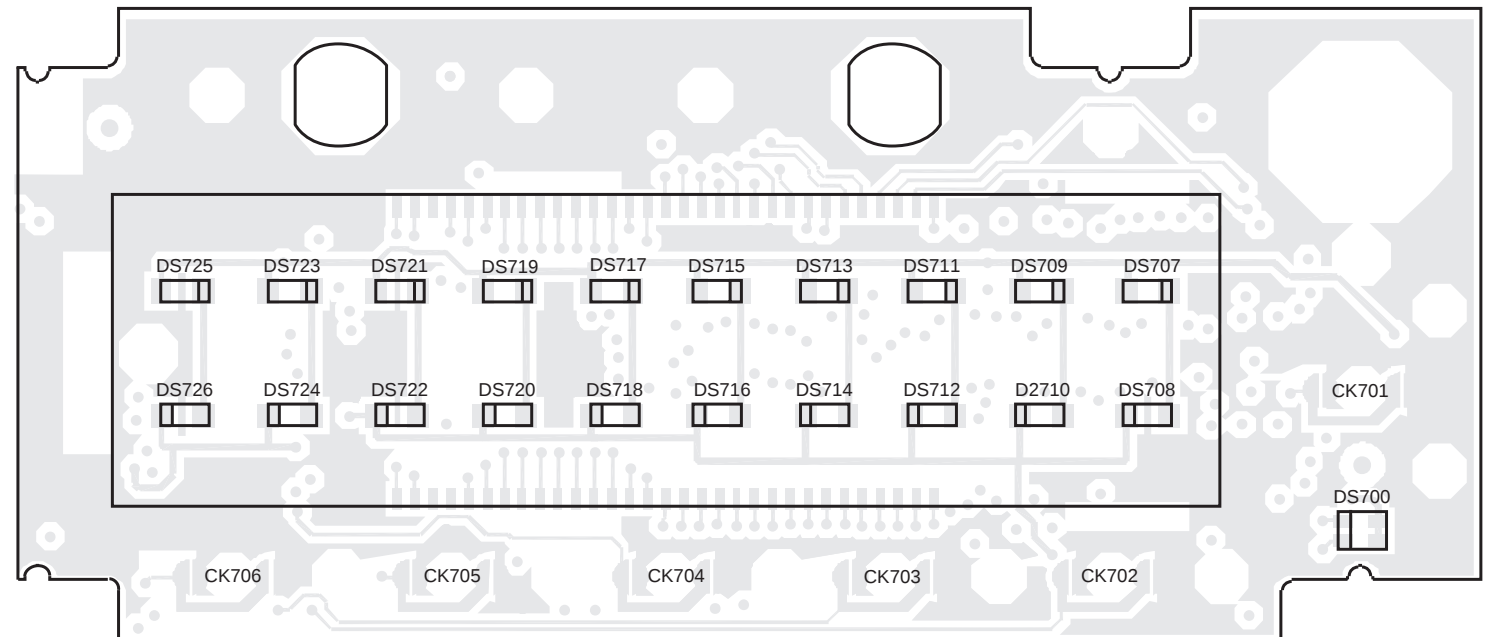
DISPLAY BOARD LAYOUT
