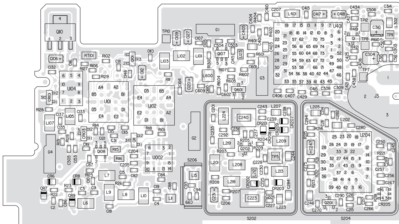
BOTTOM VIEW
