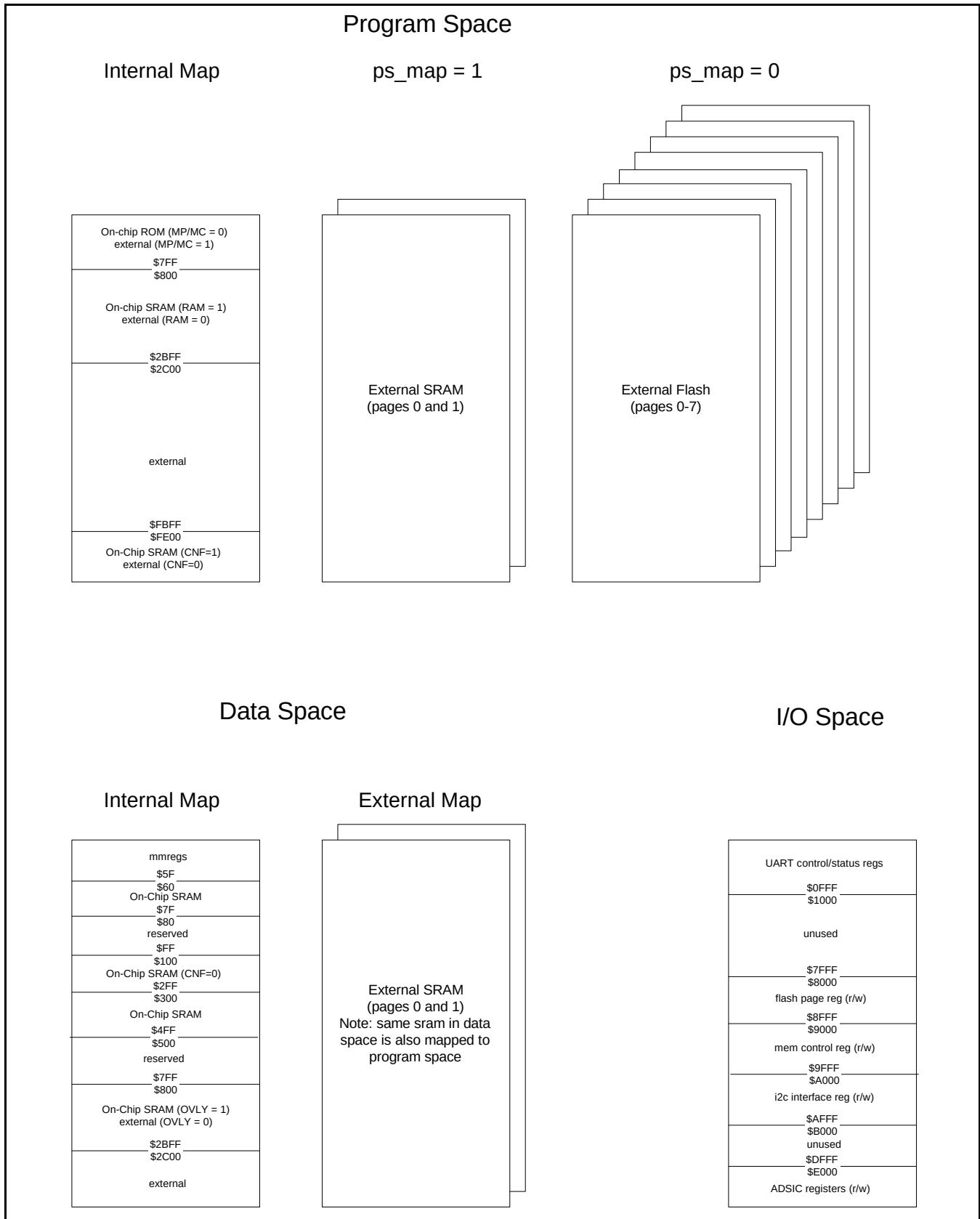
Figure 5-2 Memory Utilization
