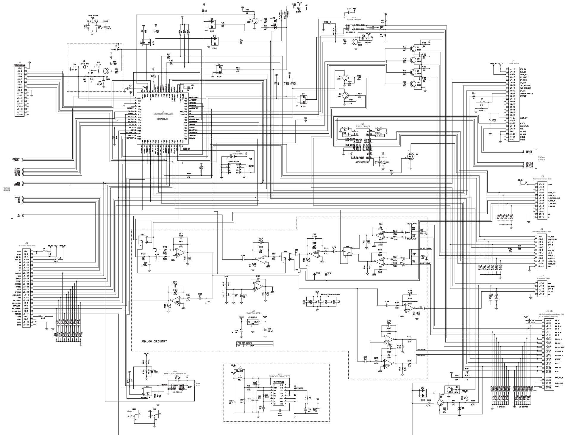
LOGIC BOARD (REV. 2) SCHEMATIC (PART 1 OF 2)
