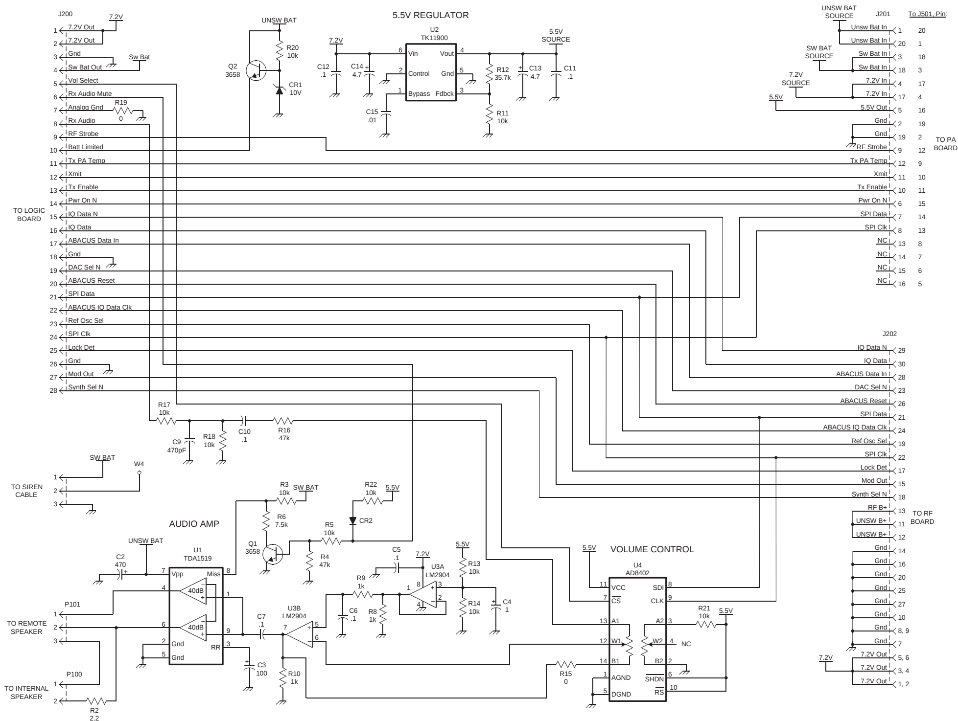
INTERFACE BOARD SCHEMATIC
