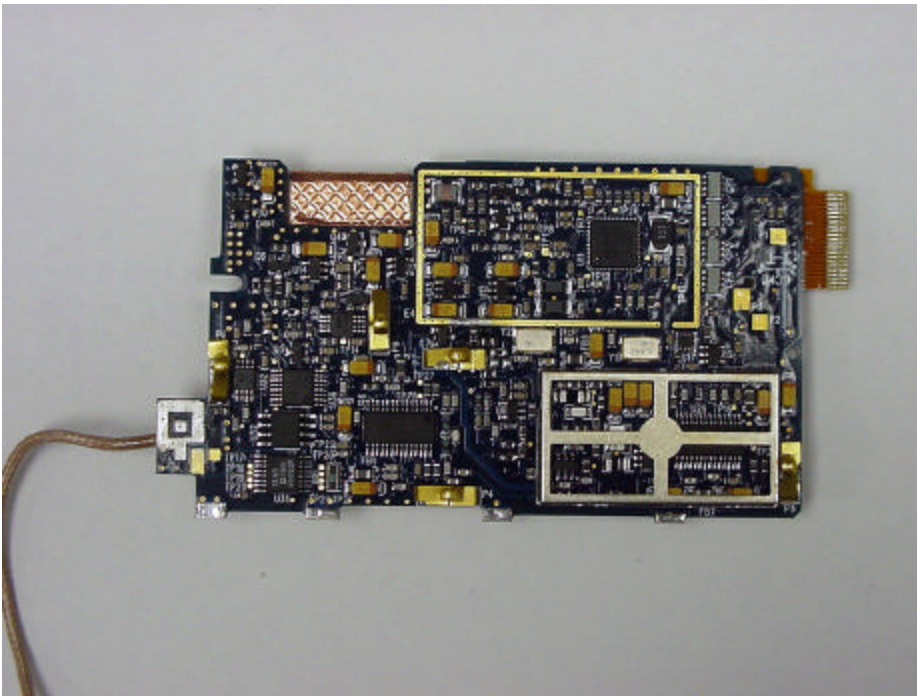
RF module bottom view without shields
