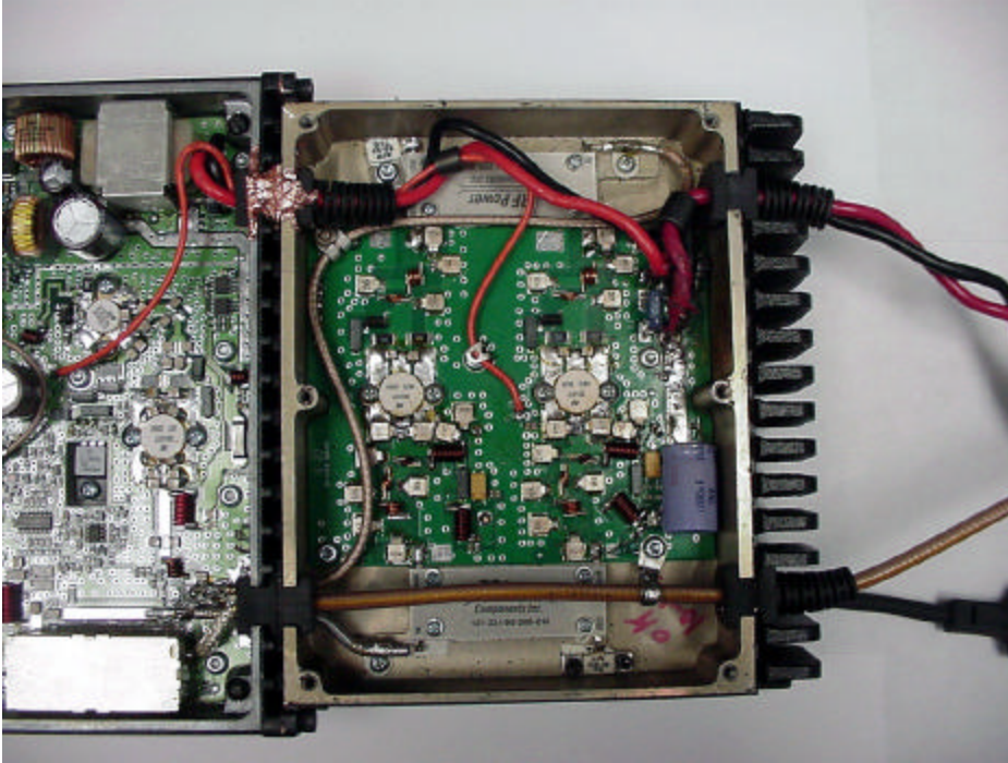
Radio top view with PA cover removed
