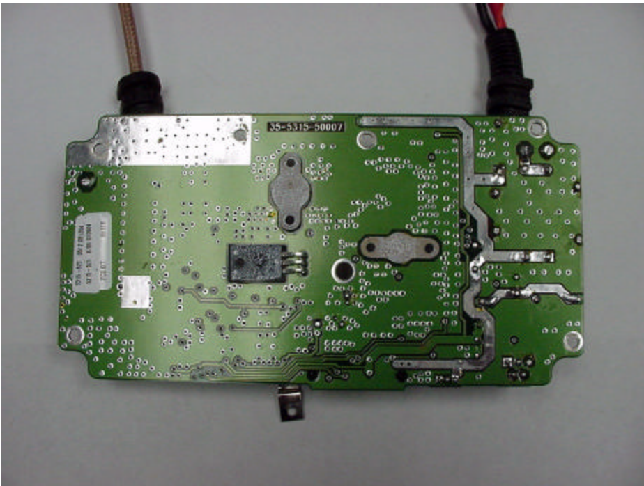
Driver PA board Bottom
