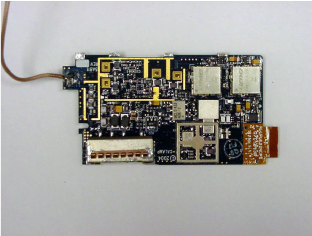
RF module top view without shields
