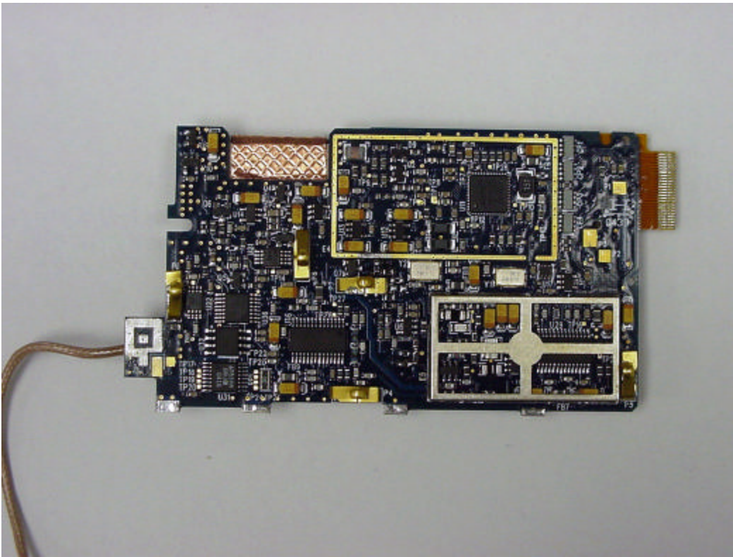
RF module bottom view without shields
