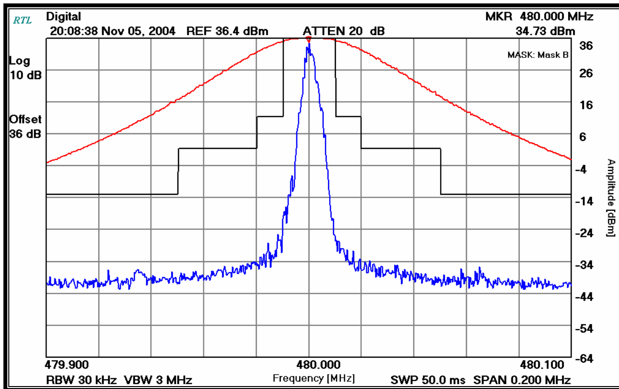
PLOT 9-3: MASK B (480 MHZ, CH 2, P25 DIGITAL)
