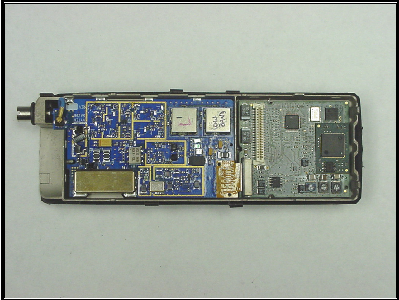
PHOTOGRAPH 29: CHASSIS WITH SHIELDS REMOVED
