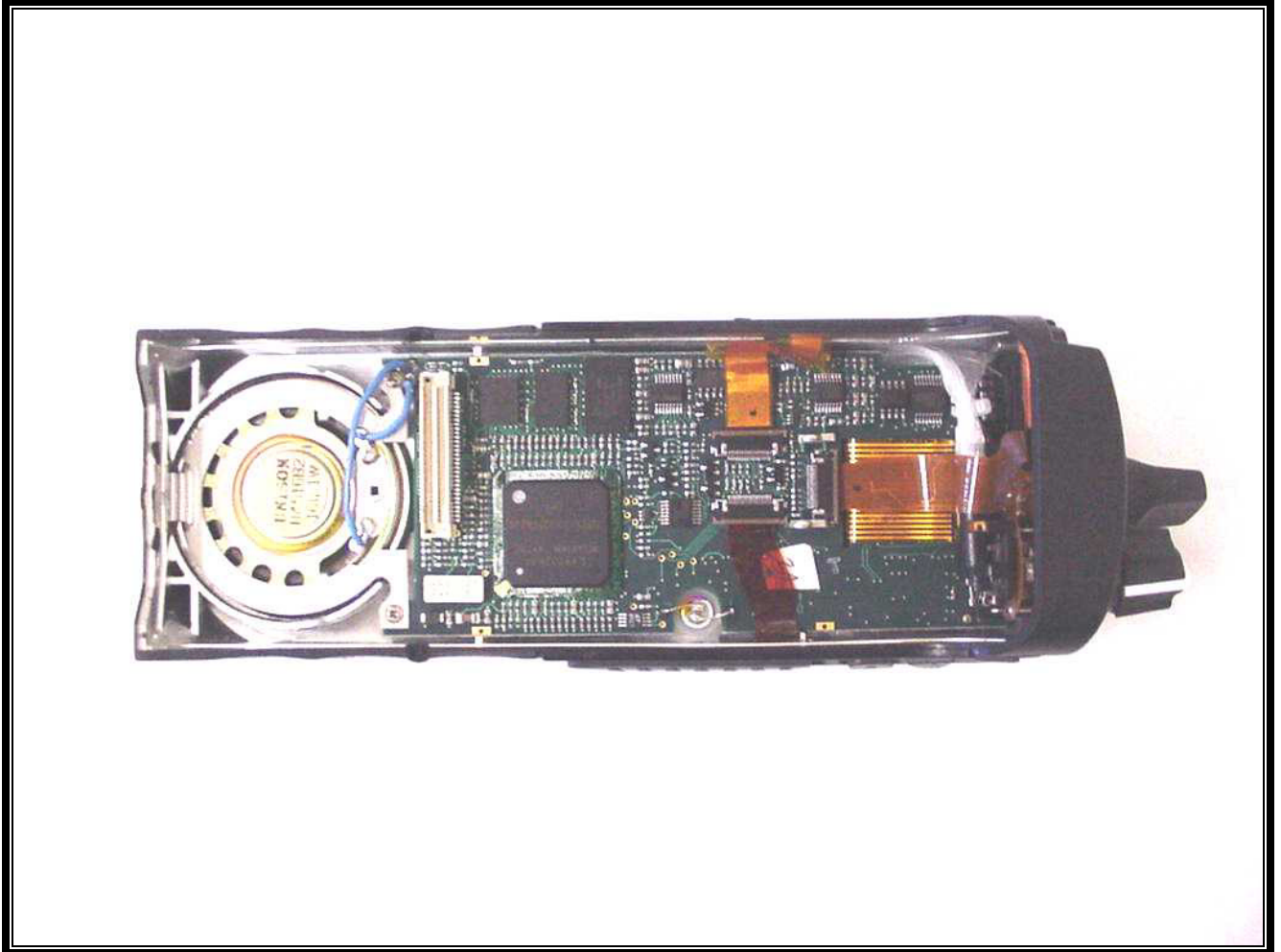
PHOTOGRAPH 35: USER INTERFACE BOARD IN FRONT COVER
