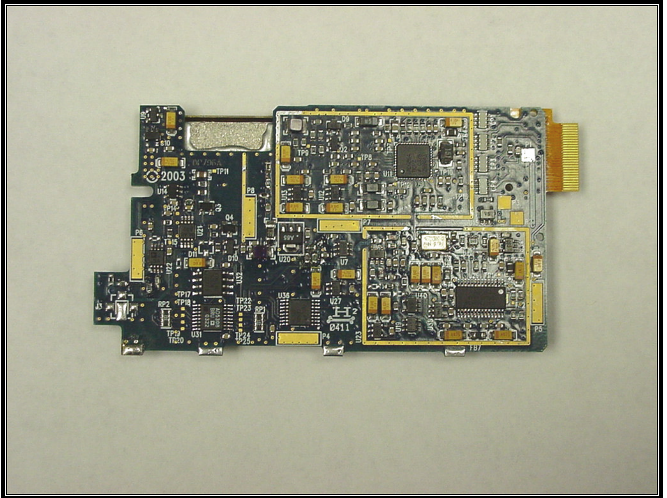
PHOTOGRAPH 33: RF BOARD BOTTOM
