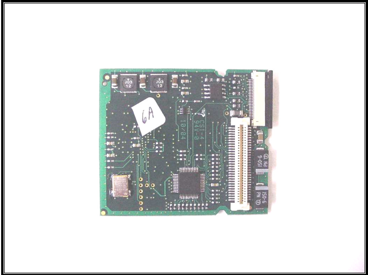
PHOTOGRAPH 32: LOGIC BOARD TOP
