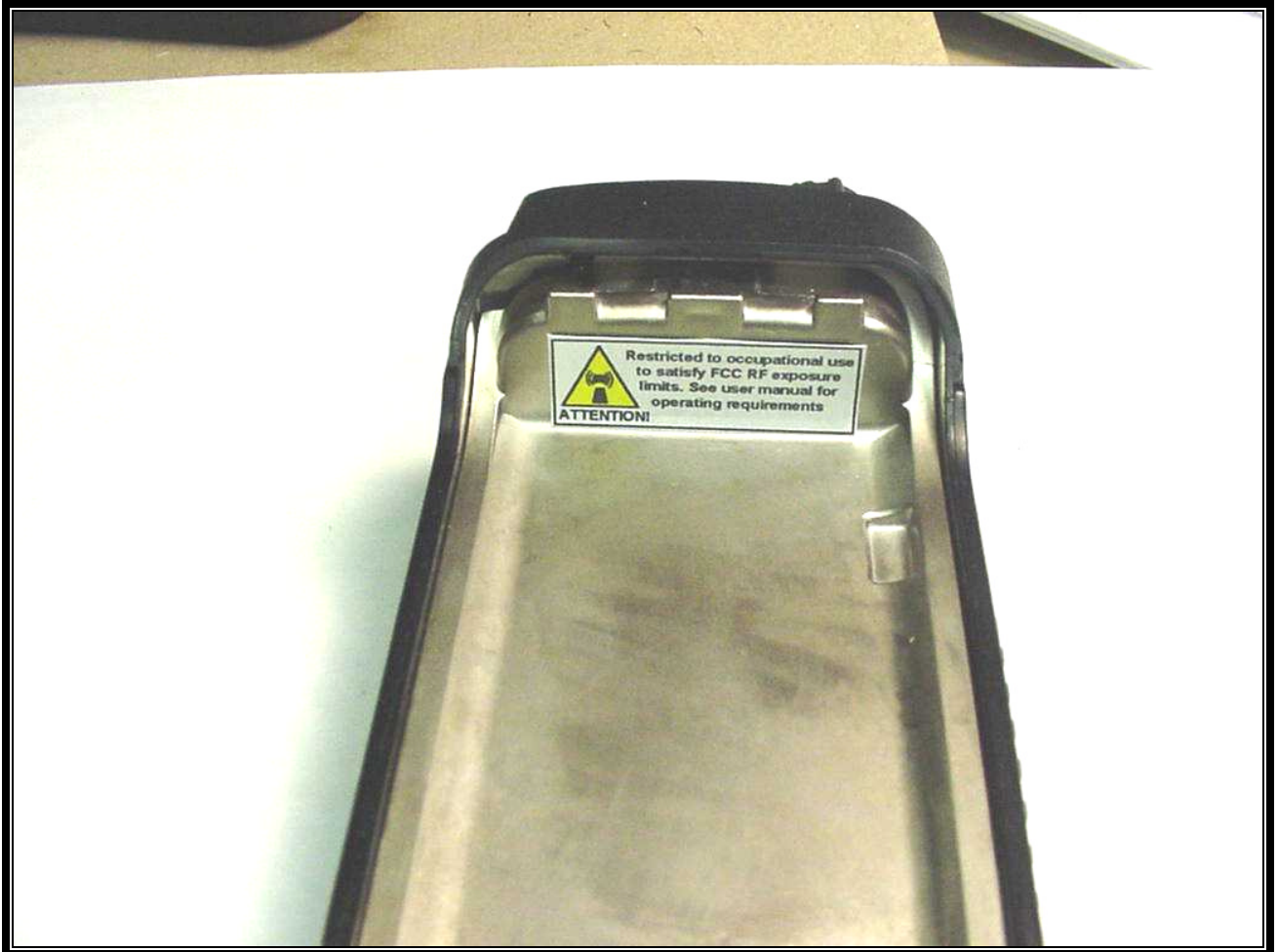
PHOTOGRAPH 2: RF LABEL AND LOCATION
