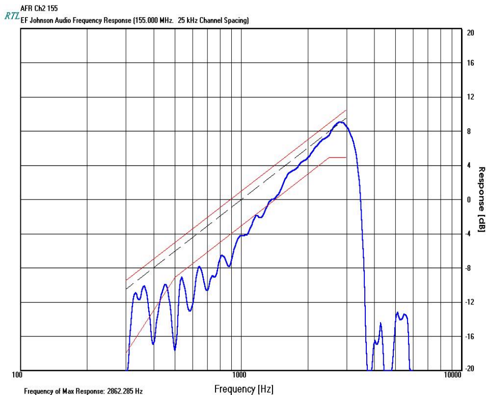
PLOT 7-1: AUDIO FREQUENCY RESPONSE – 155.0 MHZ {25 KHZ CHANNEL SPACING}
