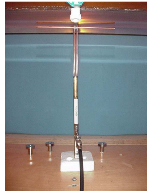
450MHz Dipole Setup
