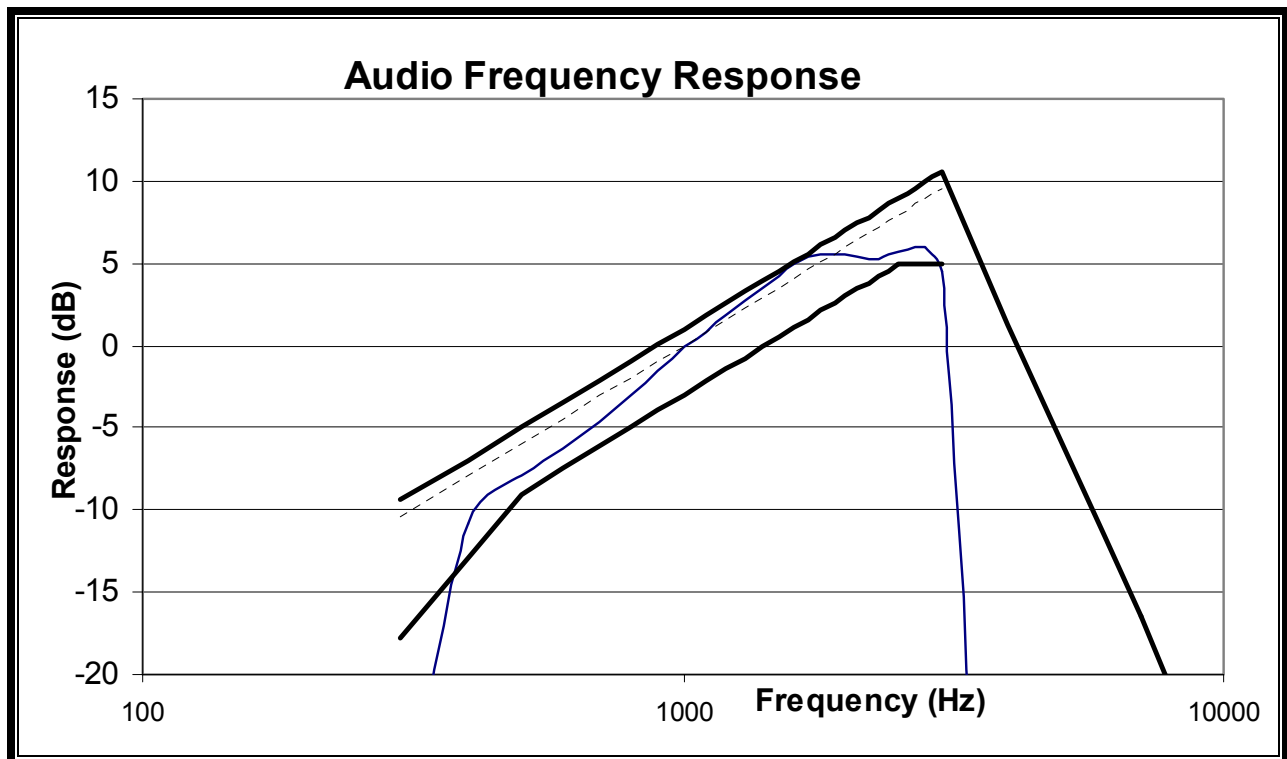
PLOT 6-1: AUDIO FREQUENCY RESPONSE
