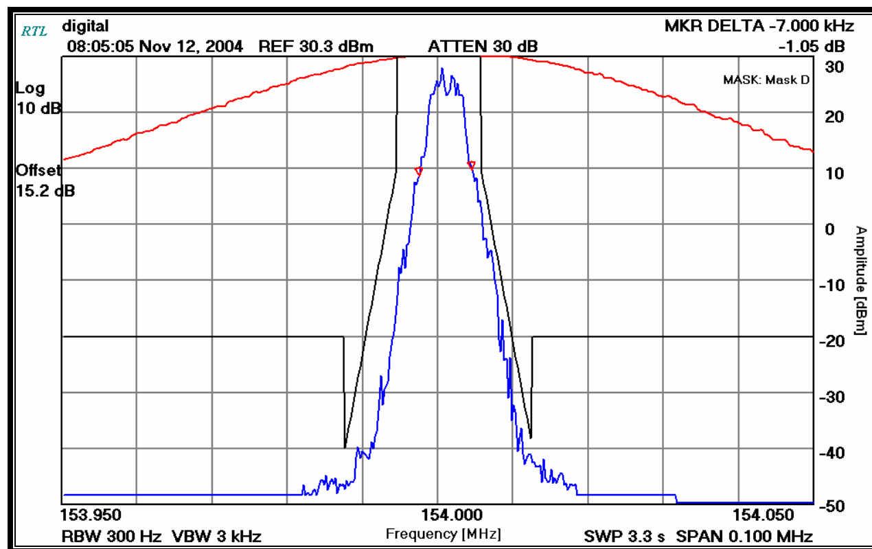
PLOT 9-1: MASK D (154 MHz; CH 8; P25 DIGITAL)
