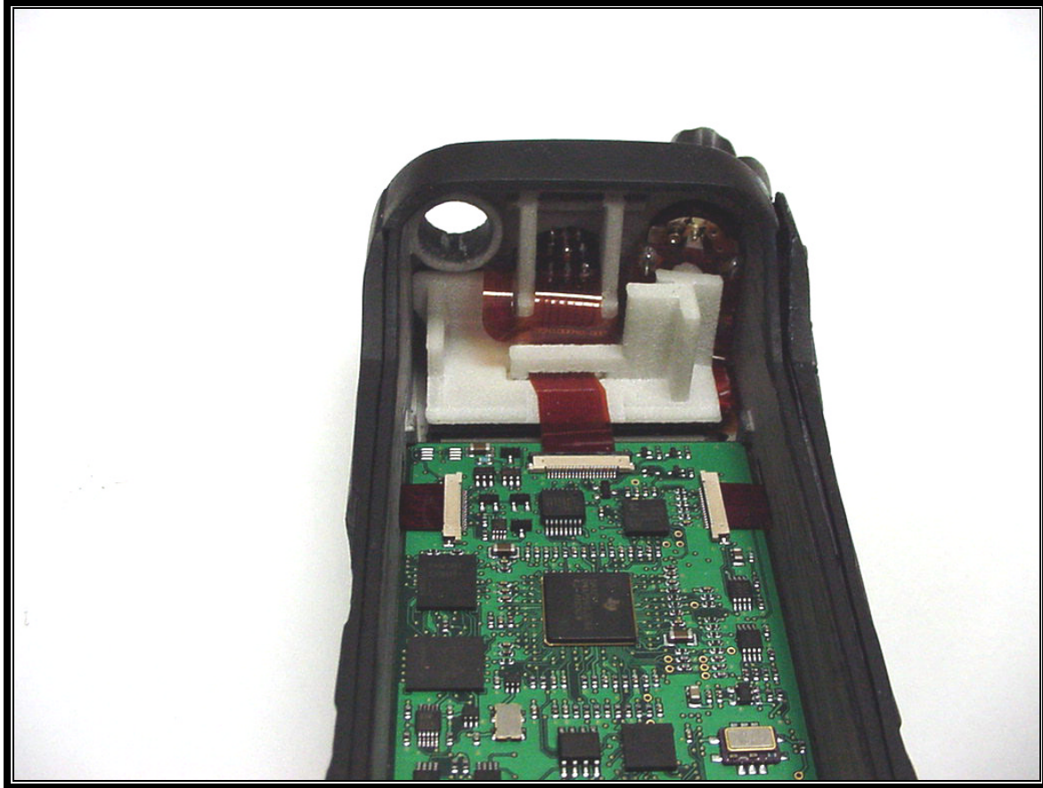
PHOTOGRAPH 19: FRONT COVER WITH DIGITAL BOARD AND CONTROL ASSEMBLY
