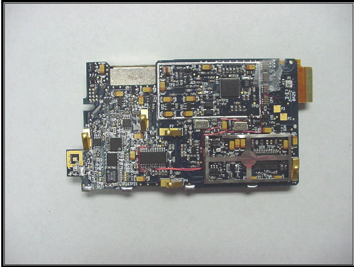
PHOTOGRAPH 16: RF BOARD BOTTOM
