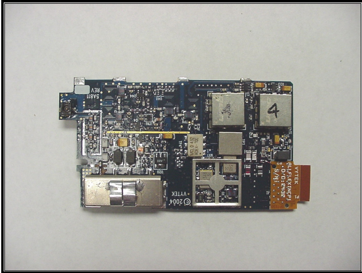
PHOTOGRAPH 17: RF BOARD TOP
