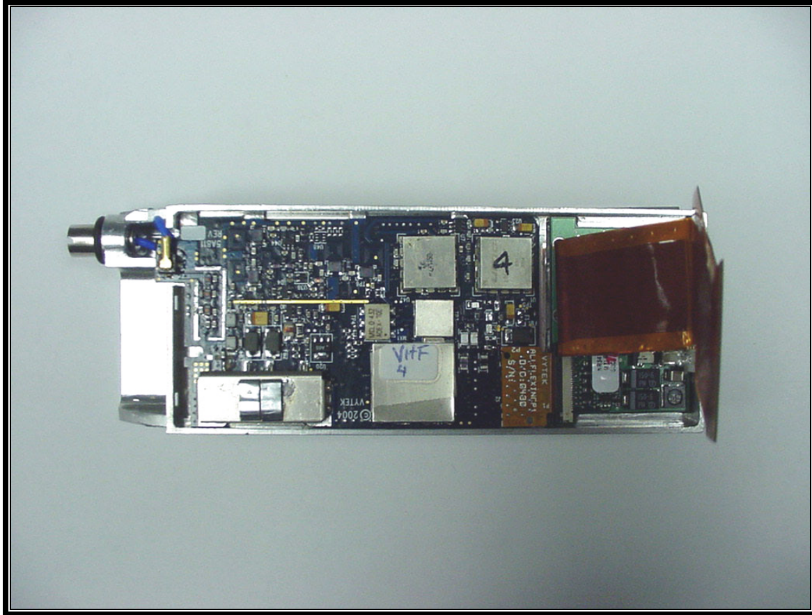
PHOTOGRAPH 13: CHASSIS WITH SHIELDS REMOVED
