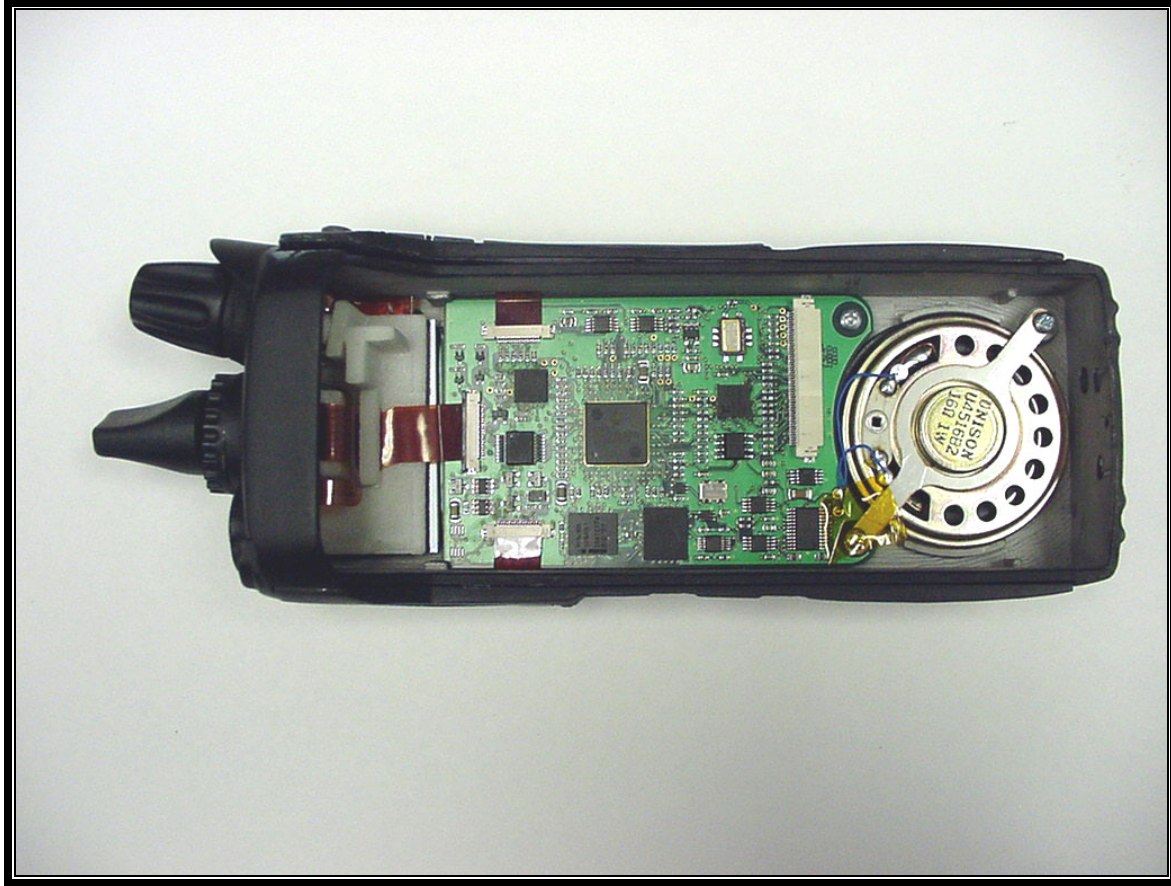
PHOTOGRAPH 18: DIGITAL BOARD IN FRONT COVER
