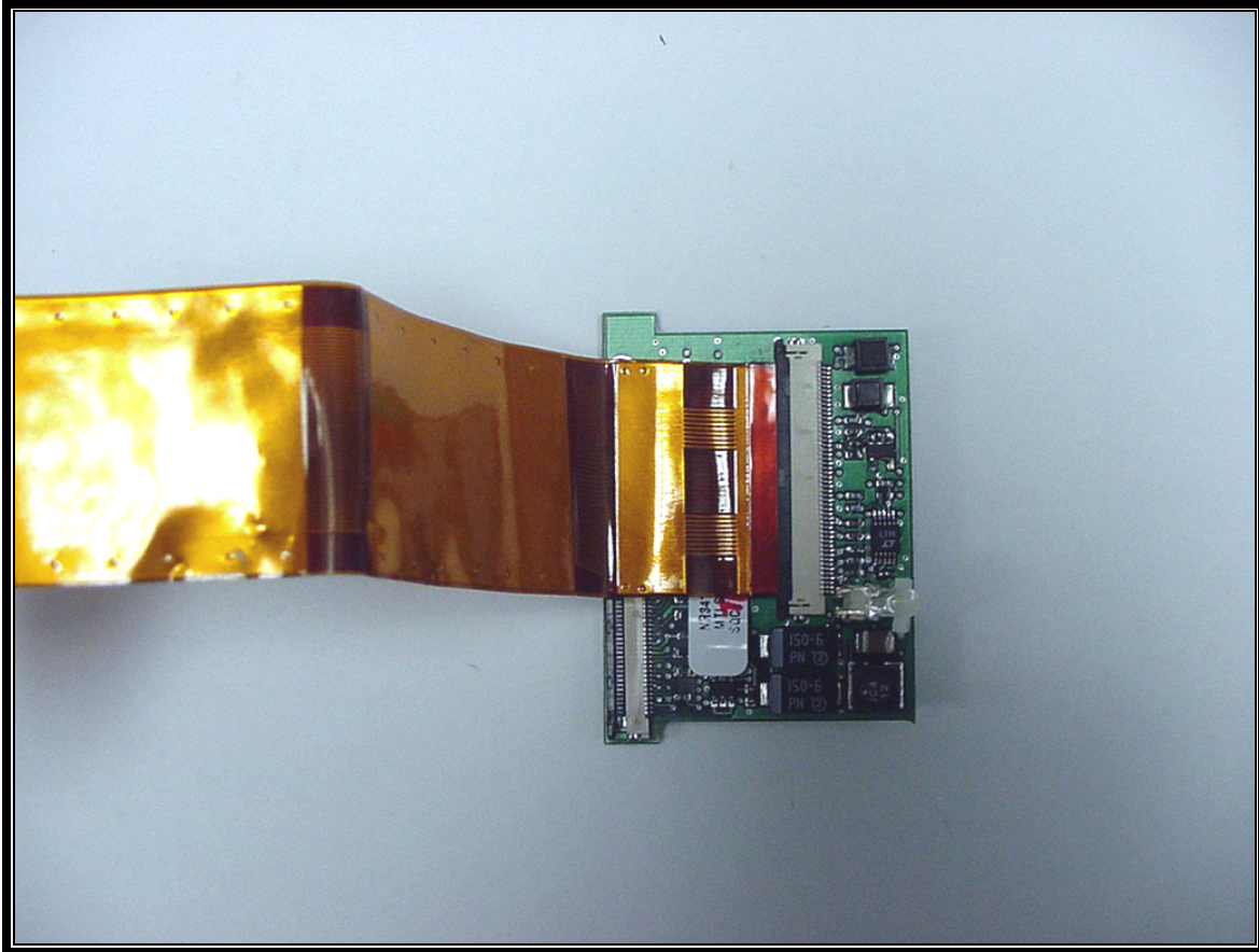
PHOTOGRAPH 14: POWER SUPPLY BOARD TOP
