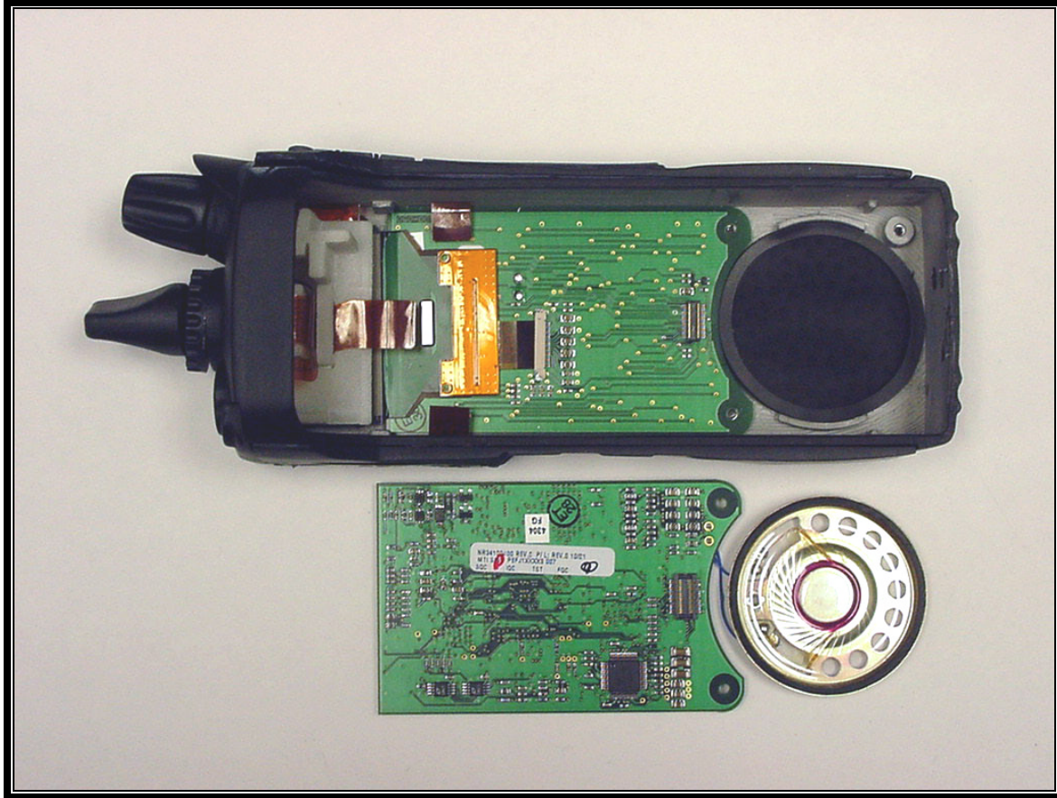
PHOTOGRAPH 20: FRONT COVER WITH DIGITAL BOARD REMOVED
