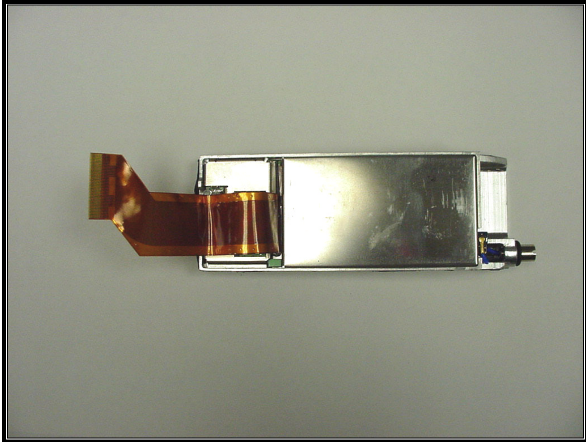
PHOTOGRAPH 12: CHASSIS WITH SHIELDS
