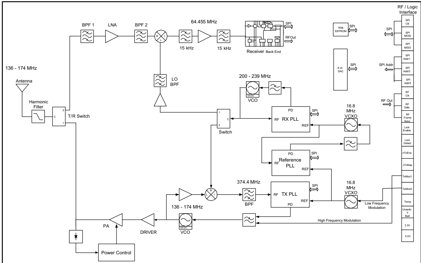
VHF RF Board Block Diagram
