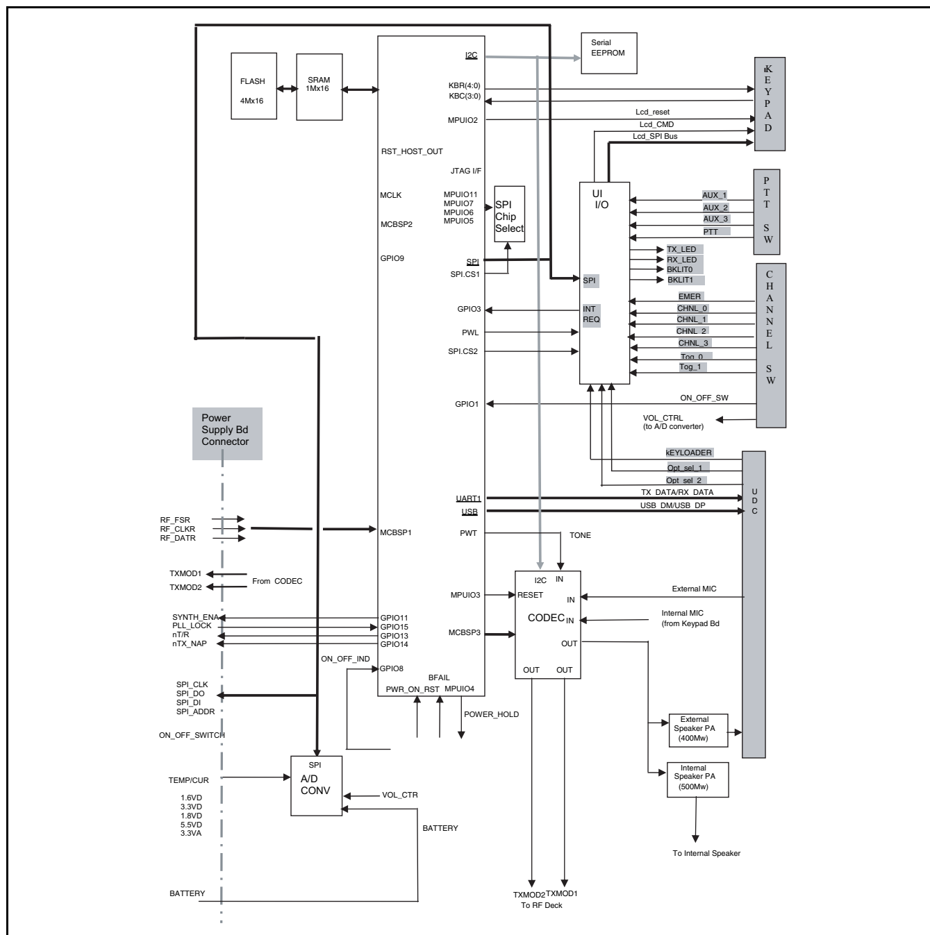
UI Board Block Diagram
