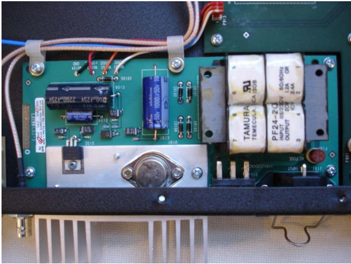
High Stability Oscillator Drawer Power Supply
