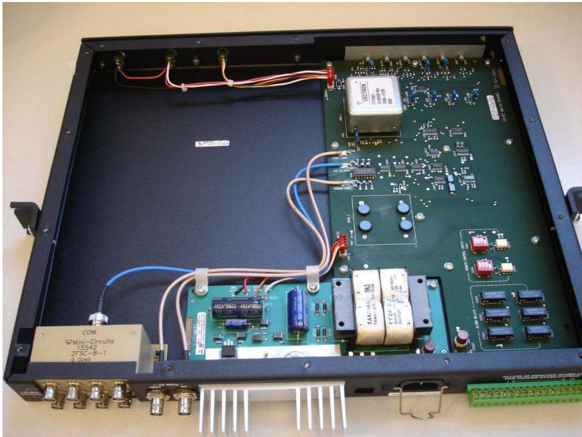
High Stability Oscillator Drawer with Cover Removed
