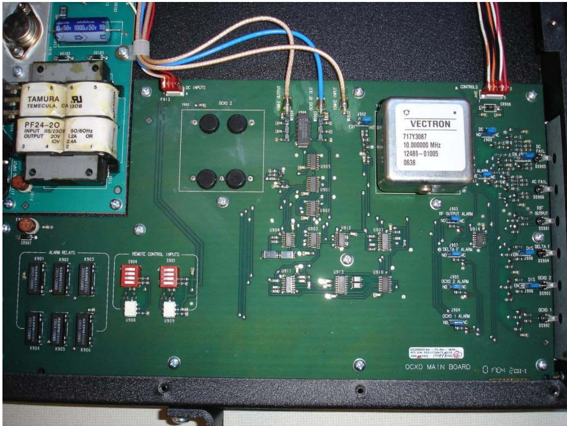
High Stability Oscillator Drawer Main PC Board Front
