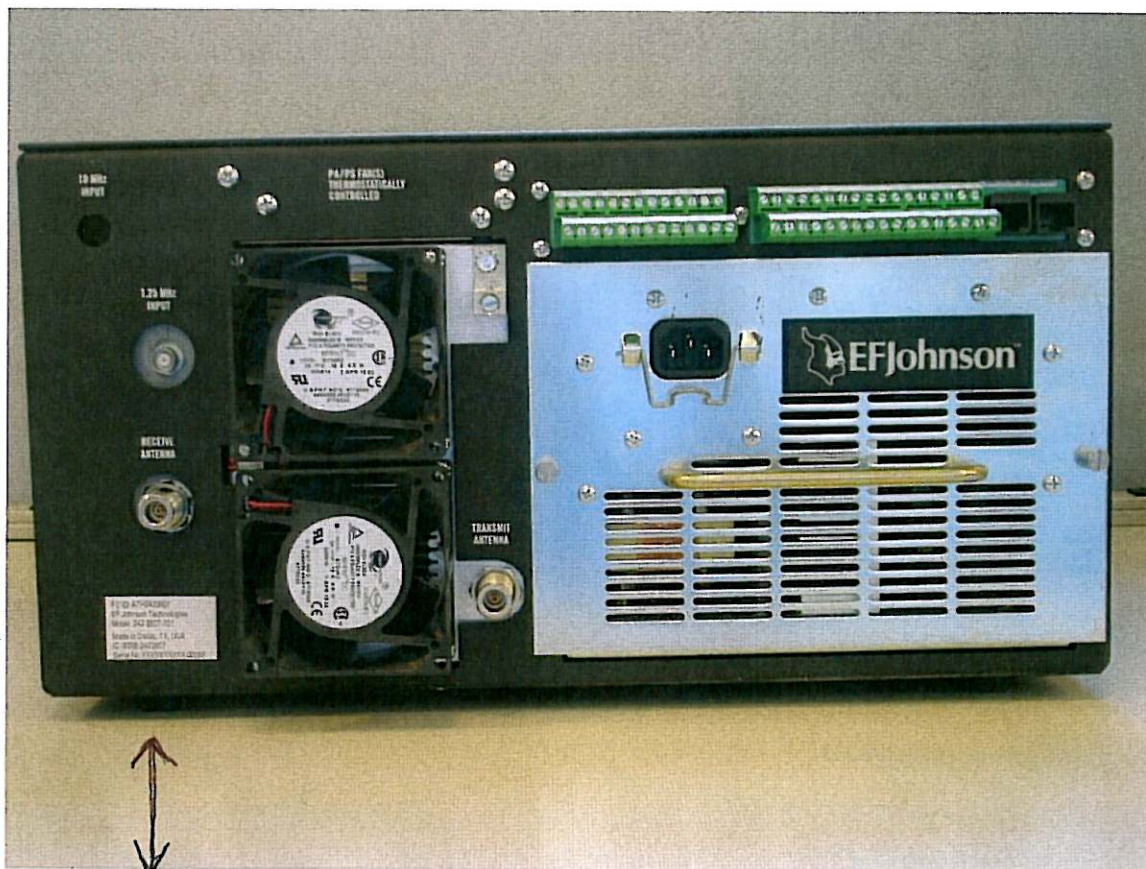
Rear View (Showing FCC/IC Label)
