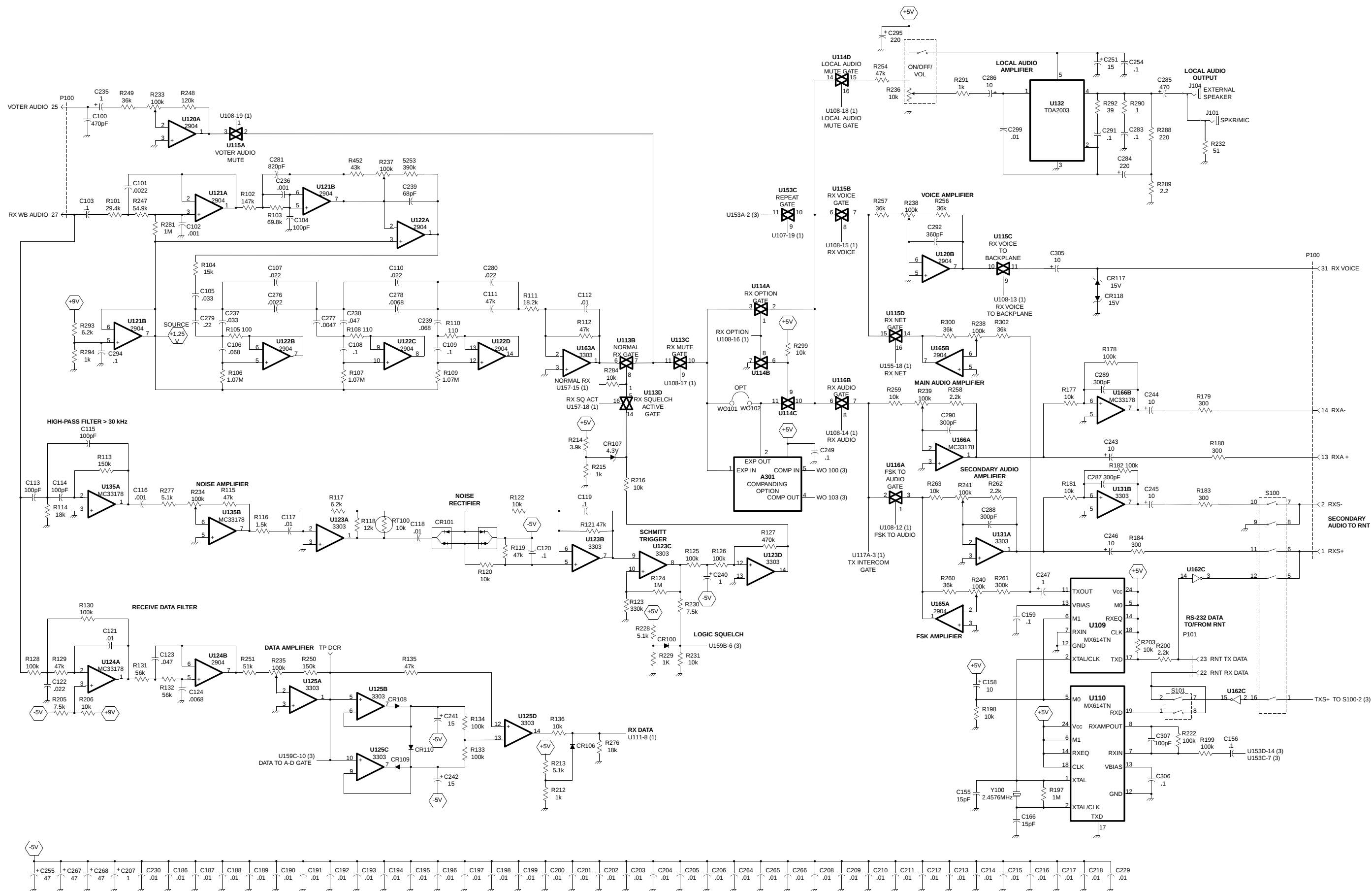
MAC SCHEMATIC (2 OF 3) FIGURE 10-28 10-24
