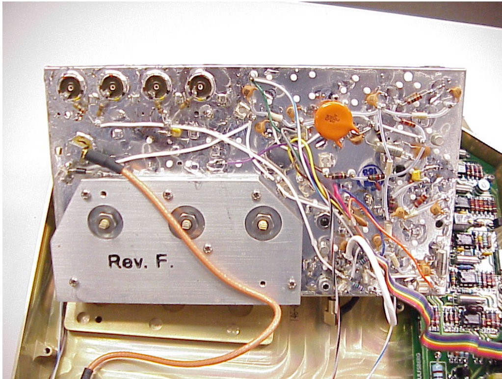
Bottom side of RT module
