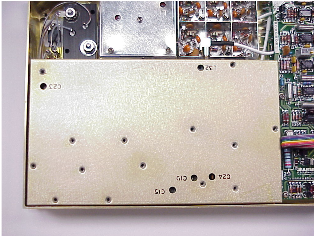
RT module with cover in place
