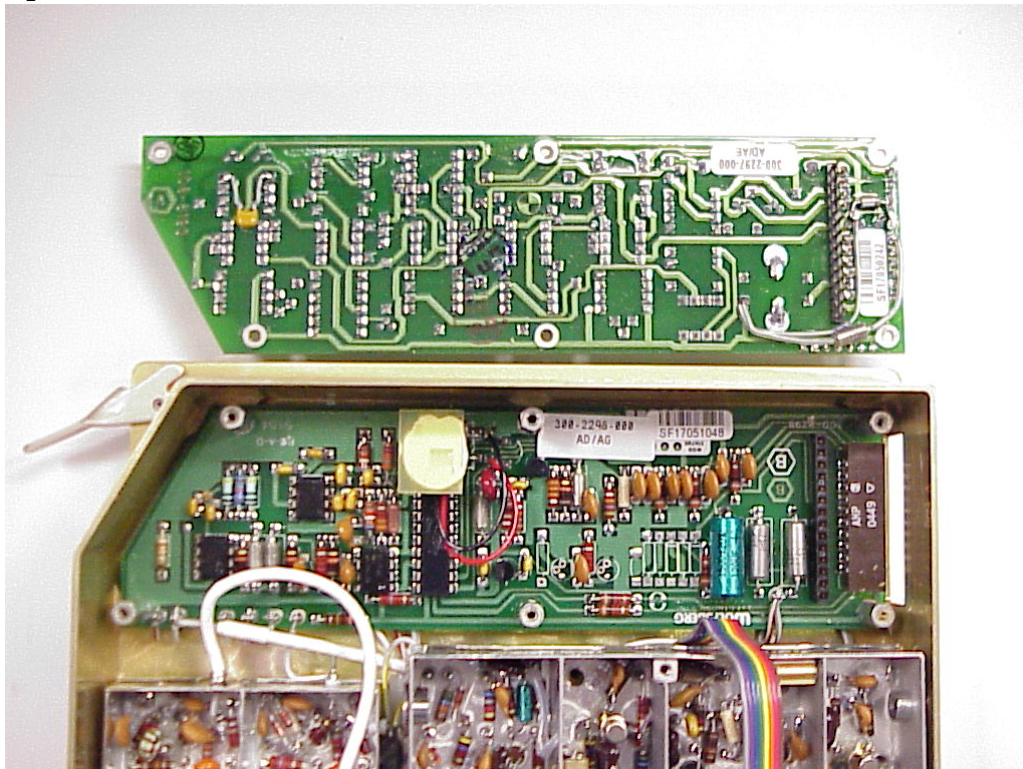
Synthesizer Bottom side
