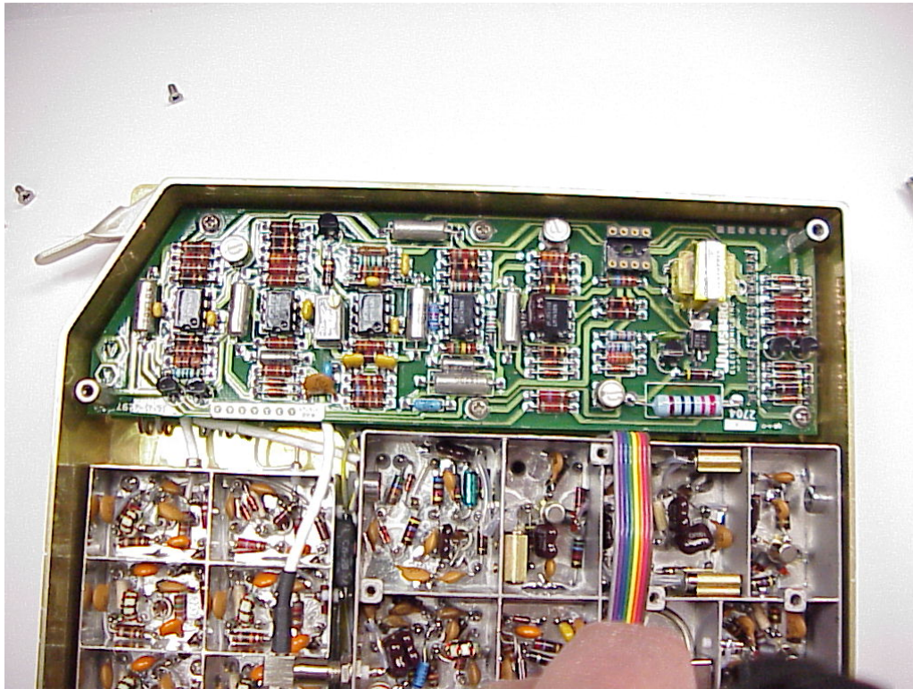
Synthesizer Top side
