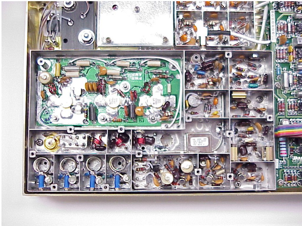
RT module with cover removed
