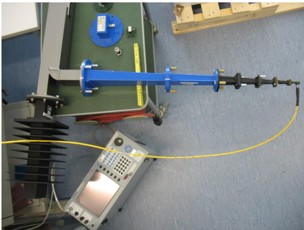
Photo No. 10: conducted measurements up to 40 GHz
