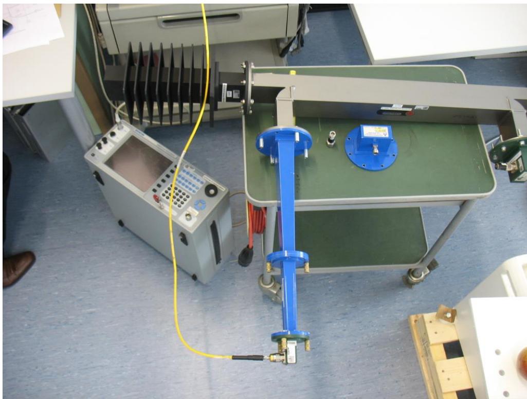
Photo No. 7: conducted measurements up to 10 GHz
