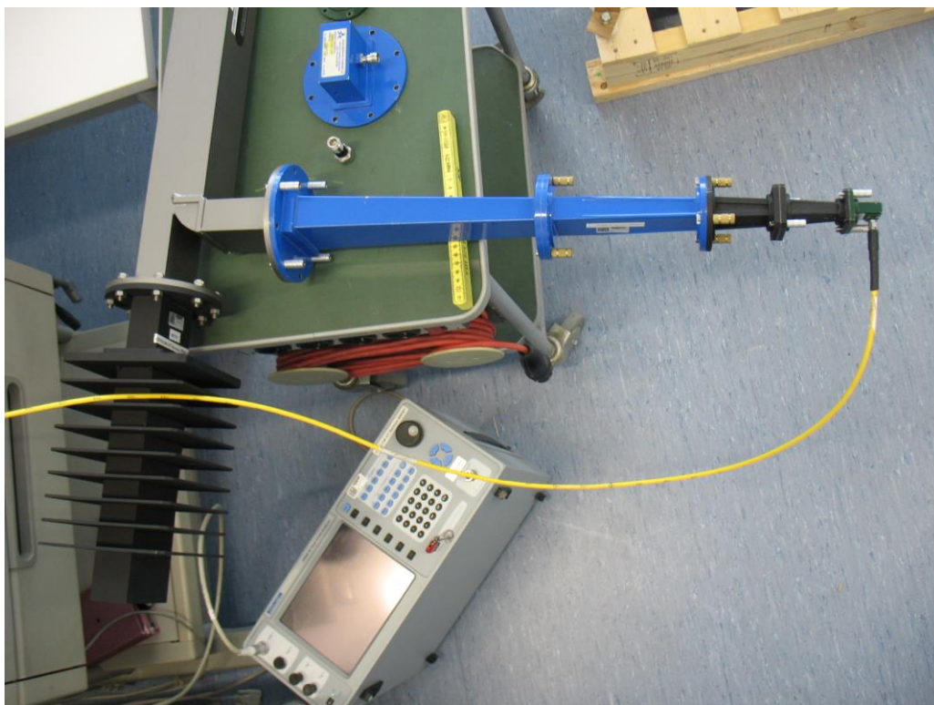
Photo No. 8: conducted measurements up to 15 GHz
