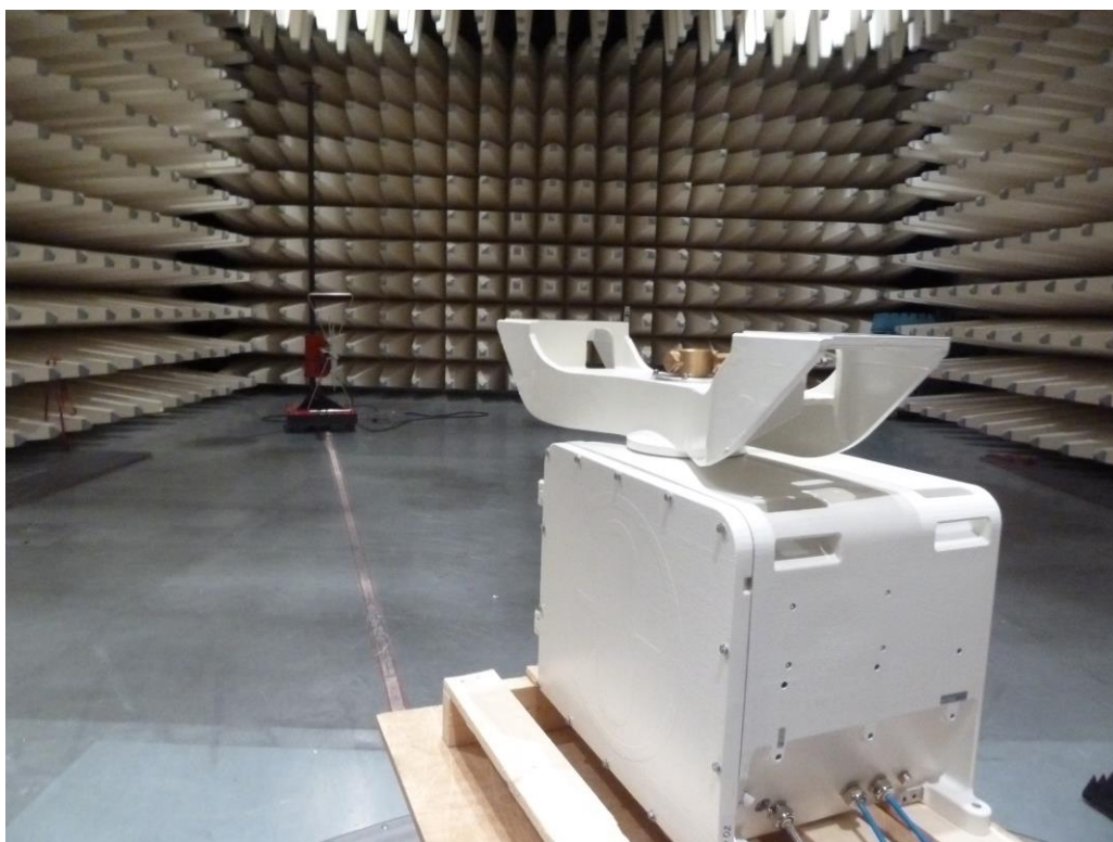
Photo No. 2: radiated spurious
