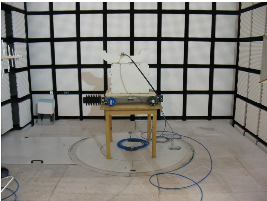
Photo No. 4: radiated spurious
