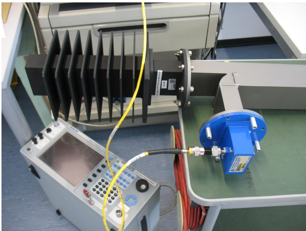
Photo No. 6: conducted measurements up to 5 GHz
