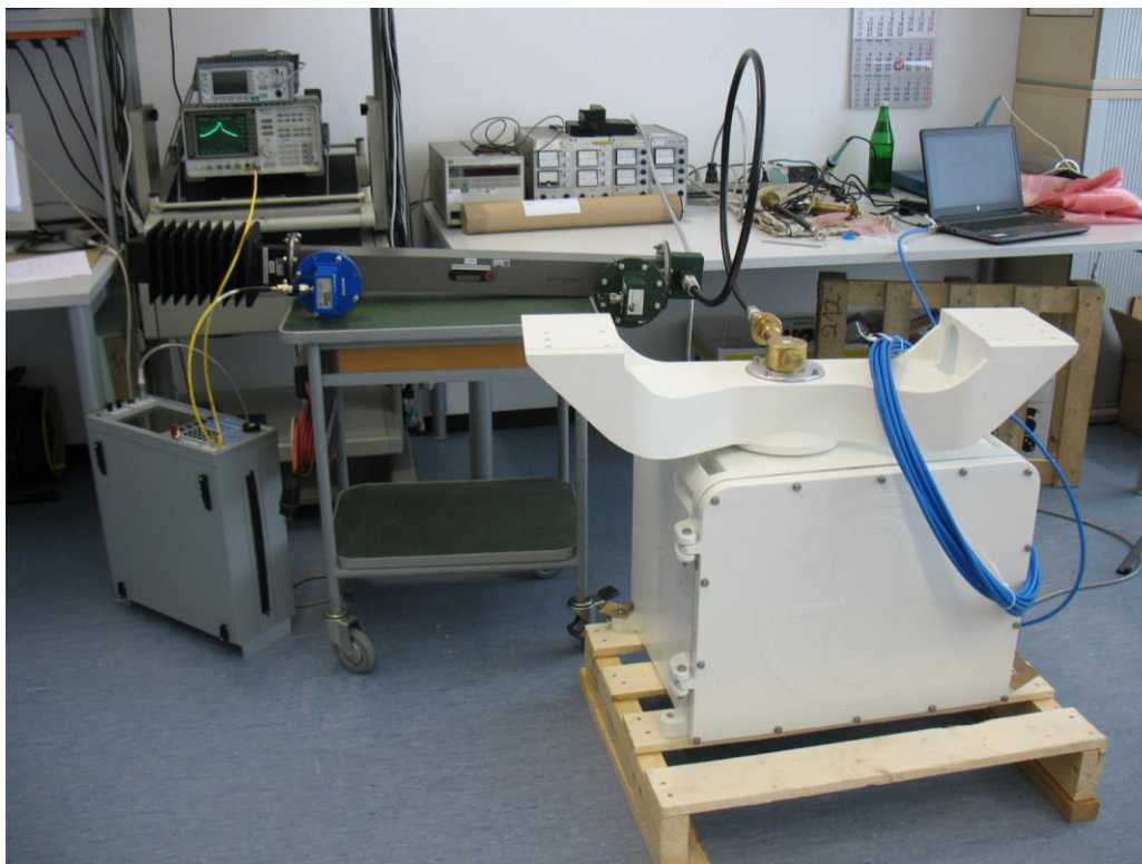
Photo No. 5: conducted measurements in test lab
