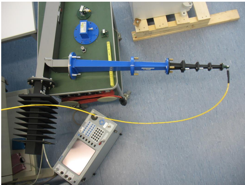
Photo No. 9: conducted measurements up to 26.5 GHz
