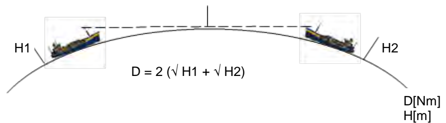
Figure 3-3 Detectable Range
