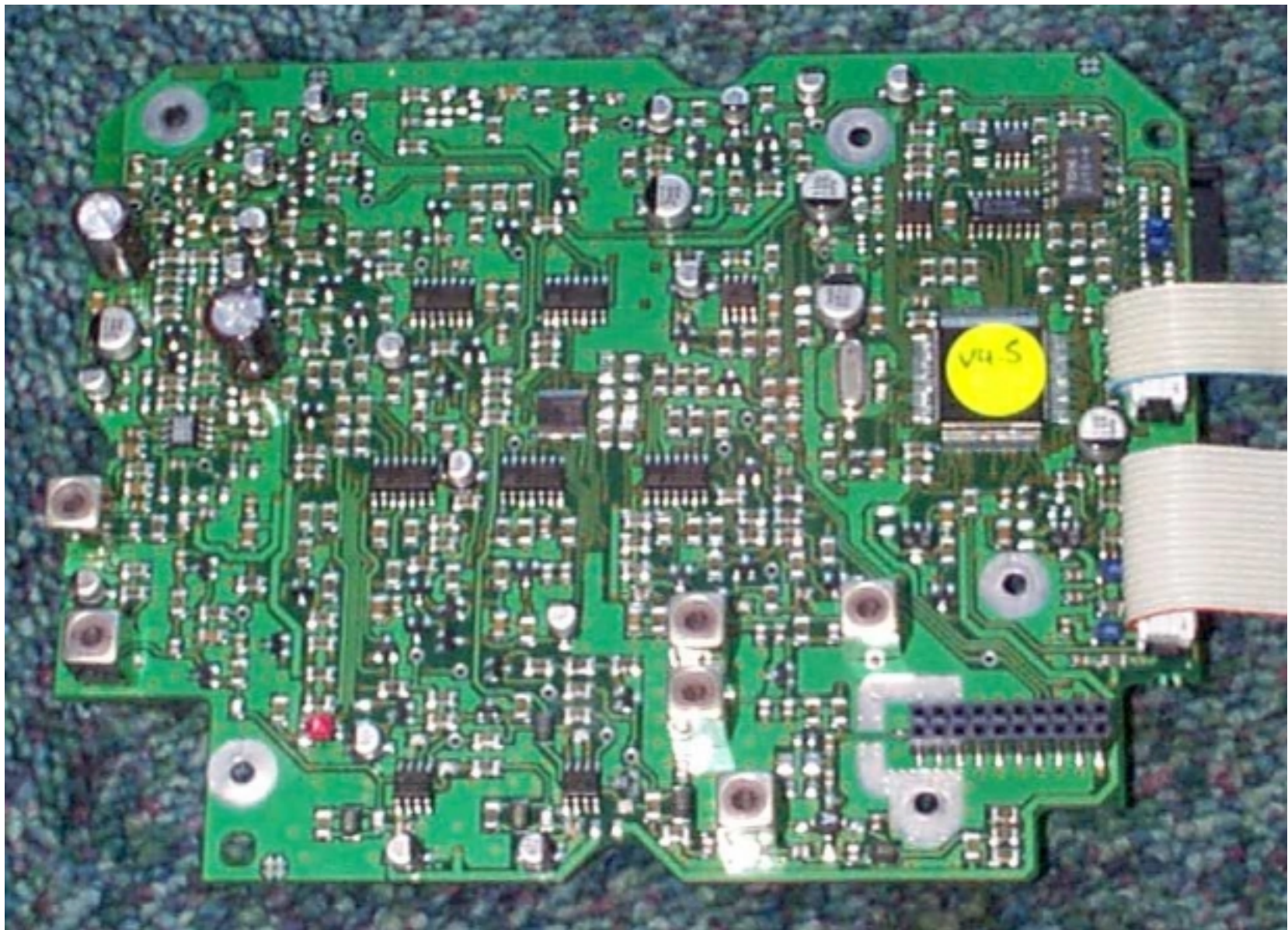
4kW, 48" Open Array Scanner Unit IF PCB
