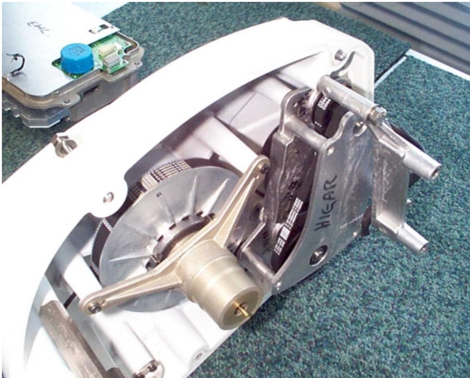
4kW, 48" Open Array Scanner Unit Gearbox and Co-axial Tube Assembly (View B)
