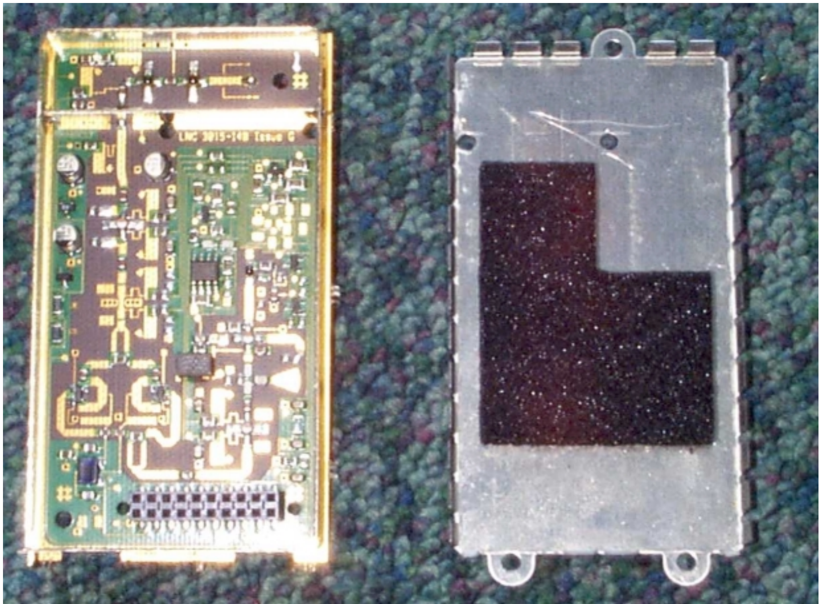
4kW, 48" Open Array Scanner Unit Low Noise Converter (LNC) Assembly and screening lid
