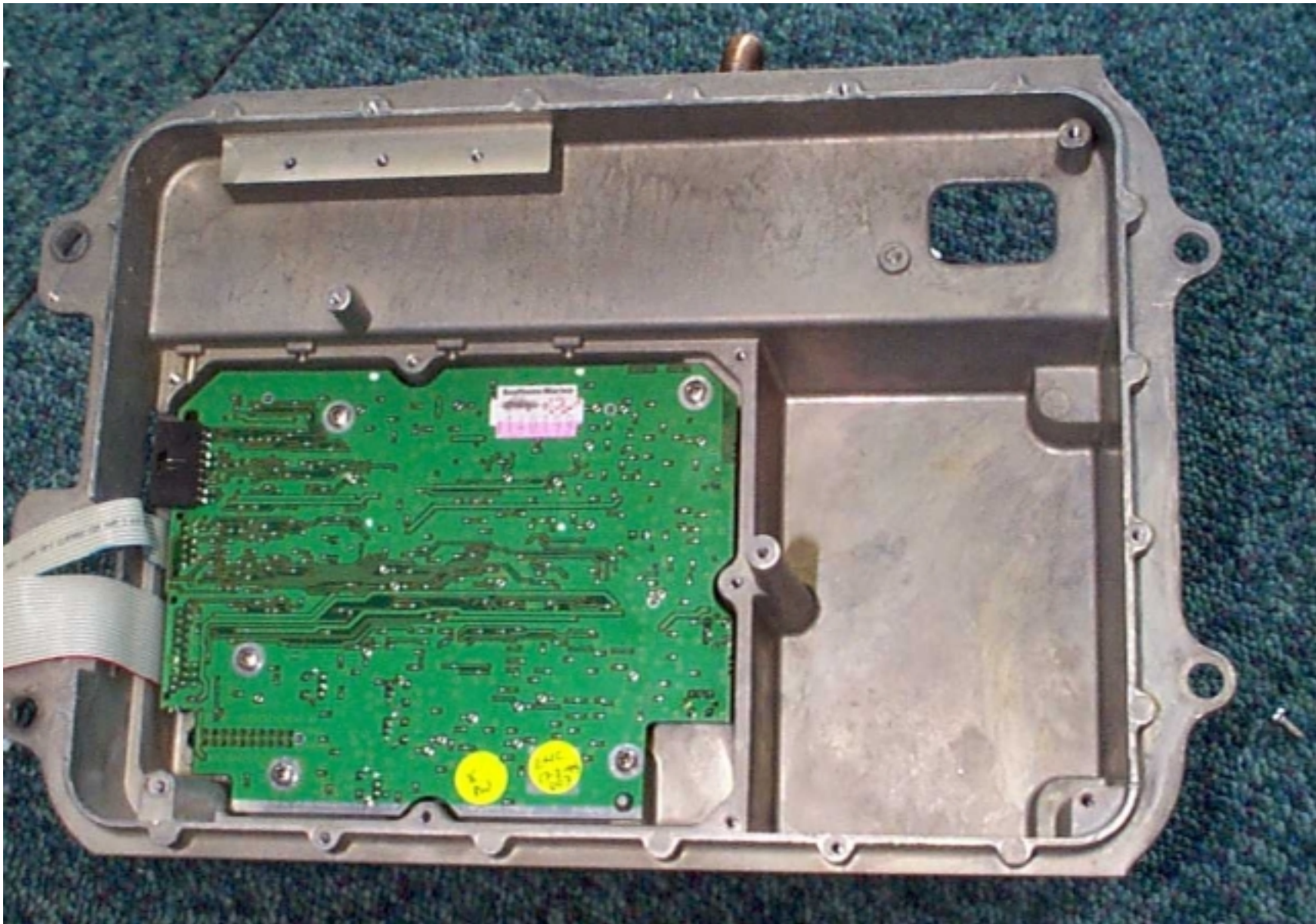
4kW, 48" Open Array Scanner Unit IF PCB – Lower view
