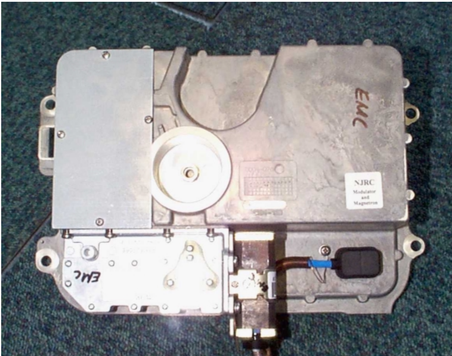
4kW, 48" Open Array Scanner Unit Core Assembly, including Magnetron and Circulator
