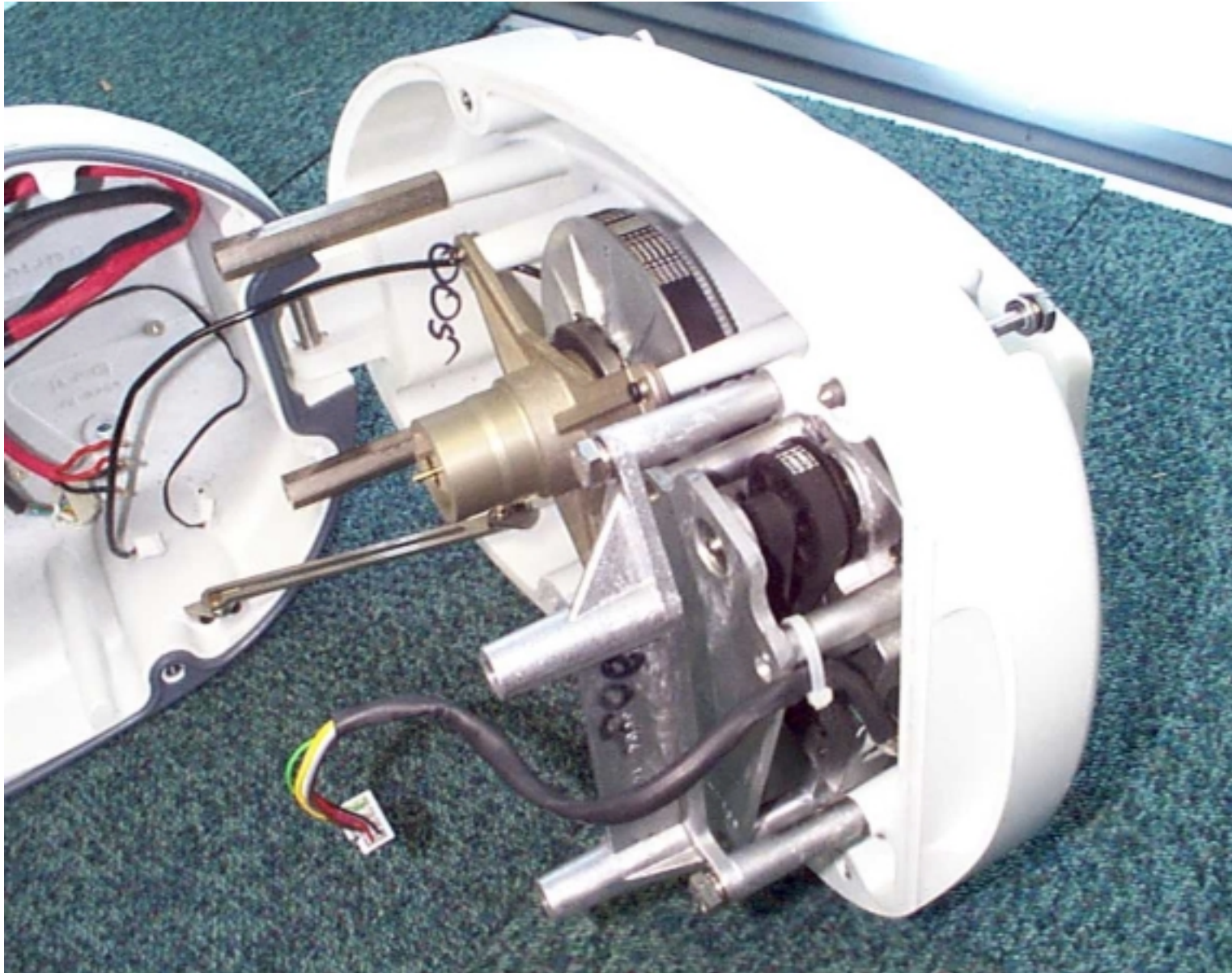
4kW, 48" Open Array Scanner Unit Gearbox and Co-axial Tube Assembly (View A)
