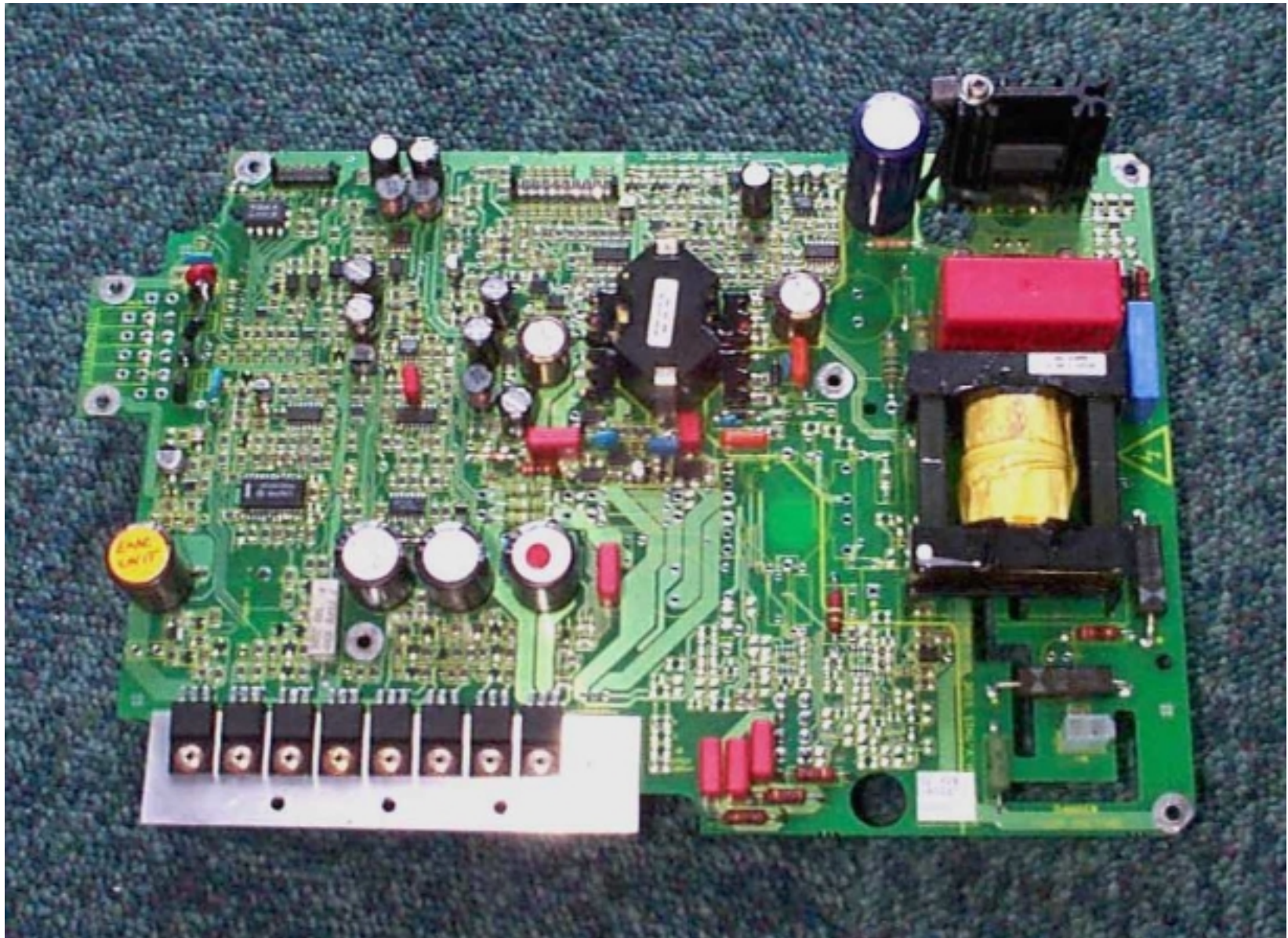
4kW, 48" Open array Scanner Unit 4kW Modulator/PSU PCB
