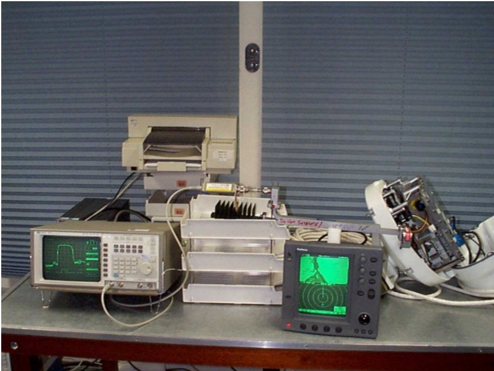
Measurements at Magnetron Port
