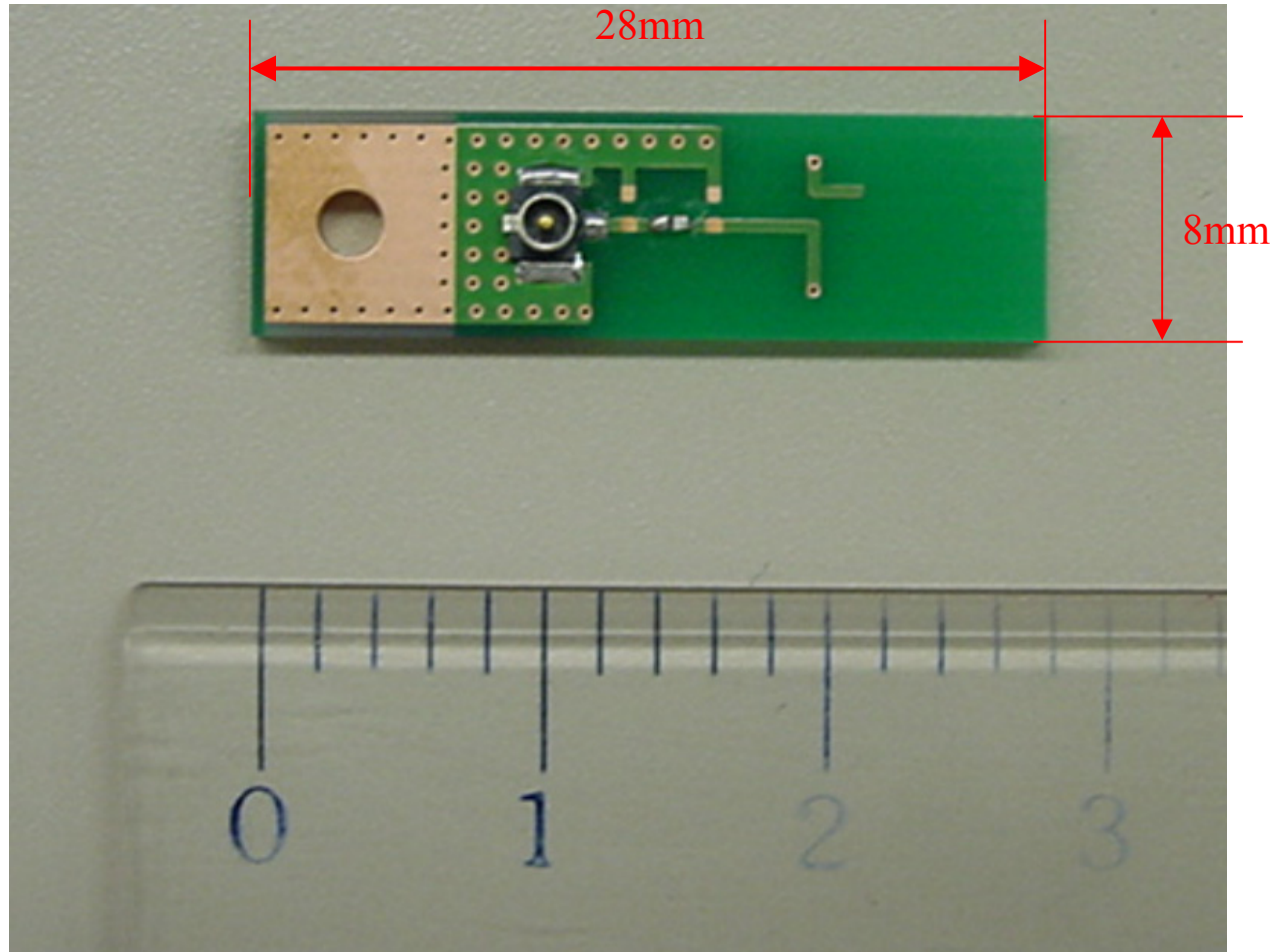
Top View
