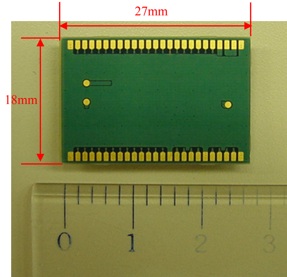
Bottom View
