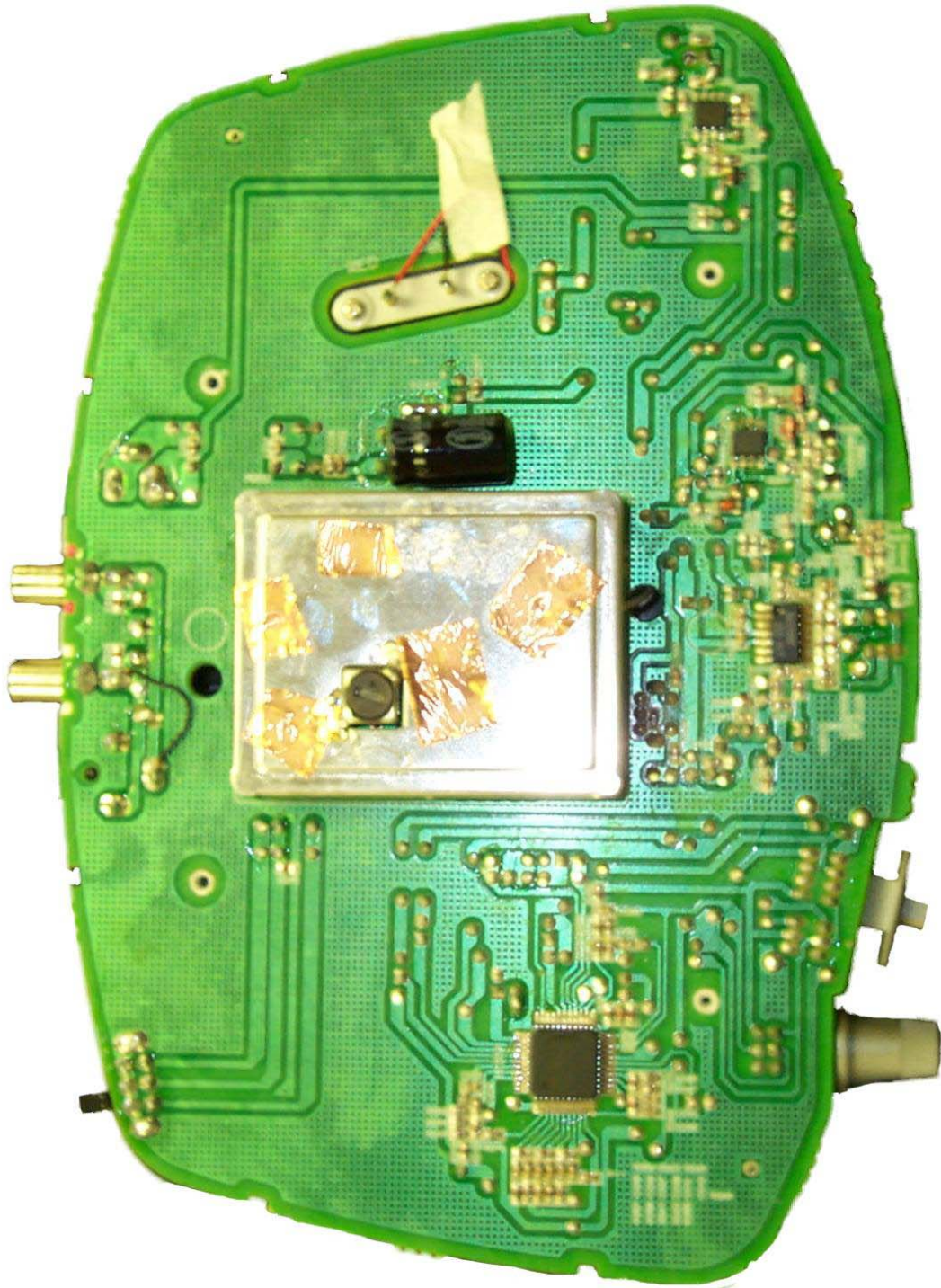
Figure 7.7 PCB Foil Side
