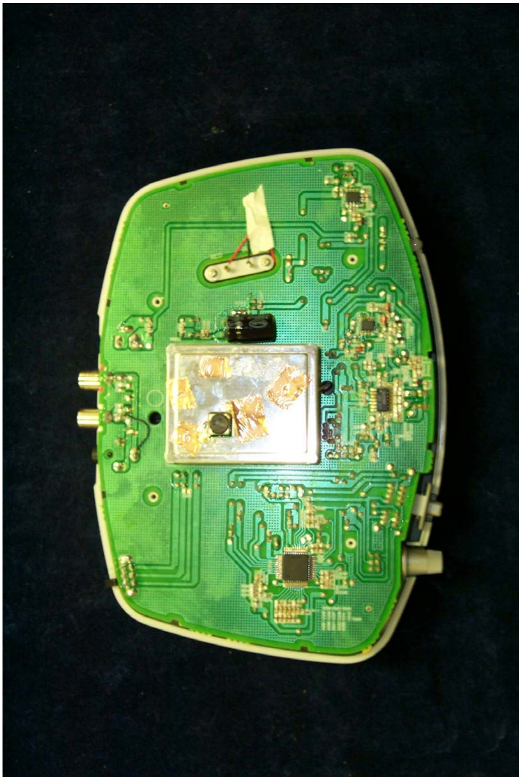
Figure 7.5 Open view
