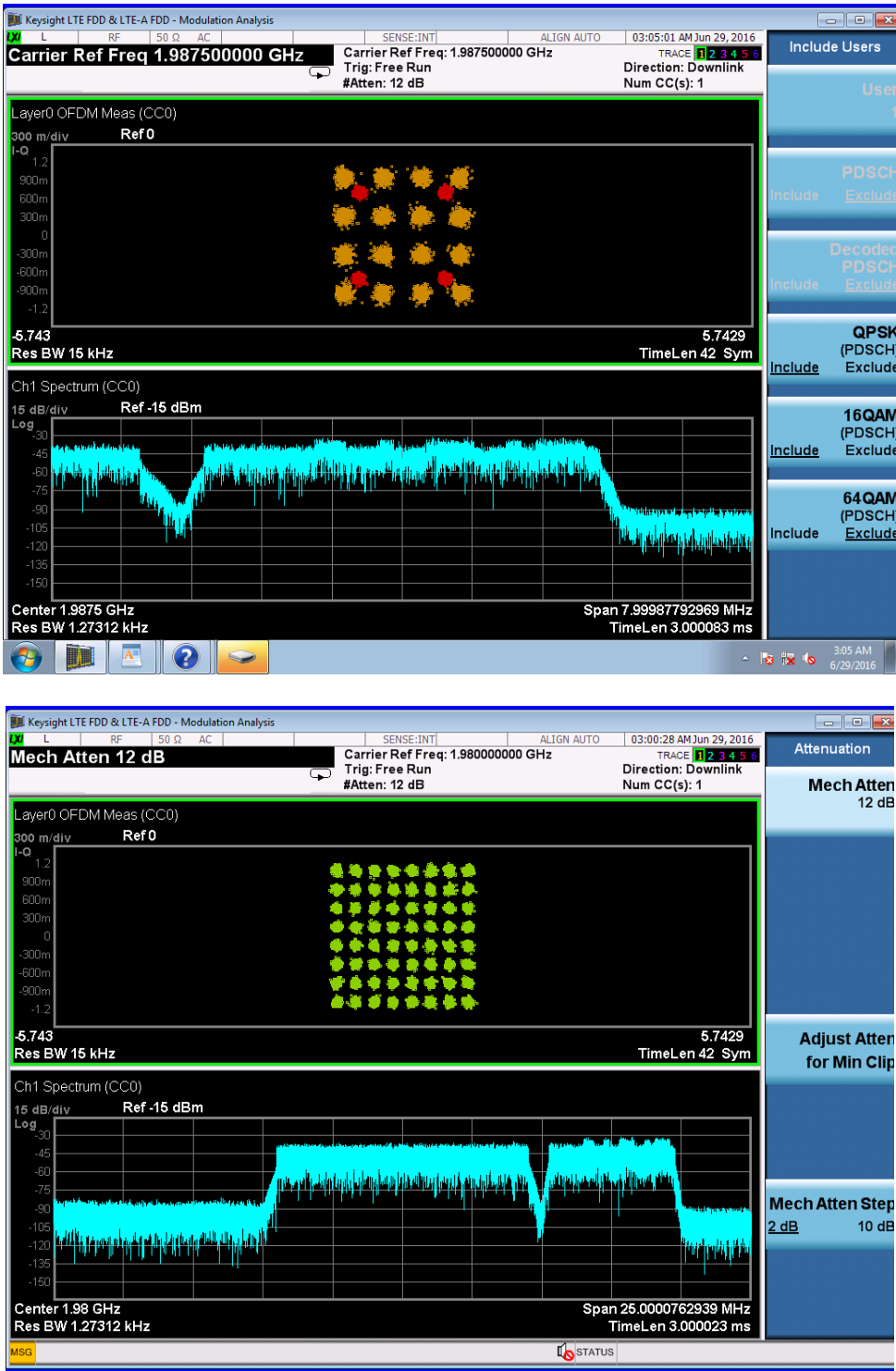
FIGURE 4.2.2 Modulation Measurement for a 5 MHz LTE Carrier at 1987.5 MHz with QPSK/16QAM AND 10 MHz LTE Carrier at 1980 MHz 64QAM Modulations
