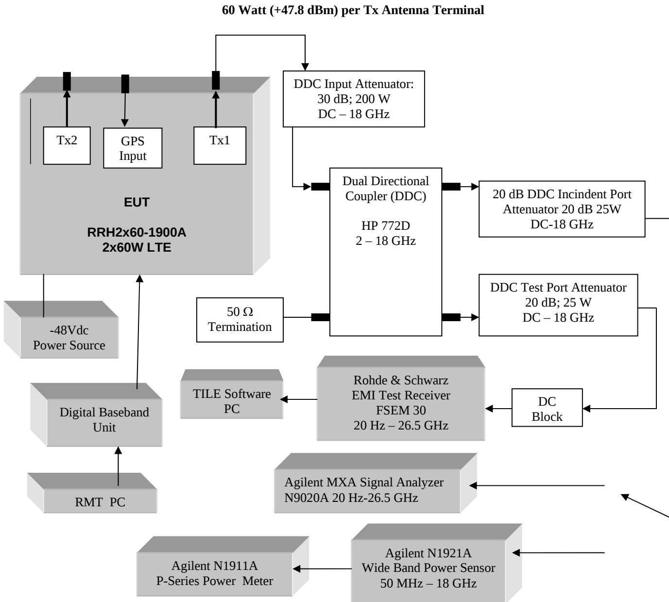
Block Diagram Of The Equipment Test Set-Up for Measurements at the Antenna Terminal
