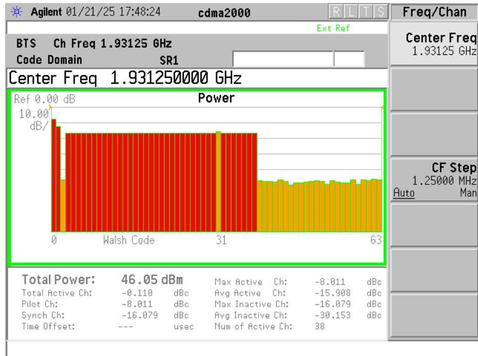
Figure 13B Typical Code Domain 1c A Block, Channel 25 Tx Output
