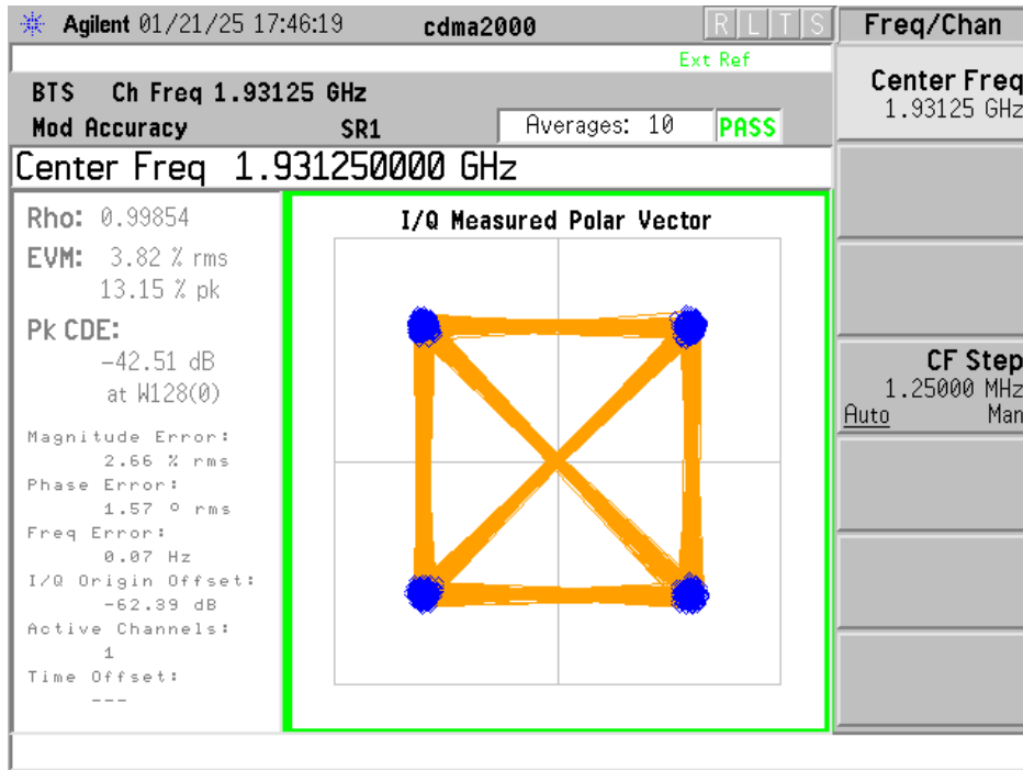
Figure 13B Typical Rho 1c A Block, Channel 25 Tx Output
