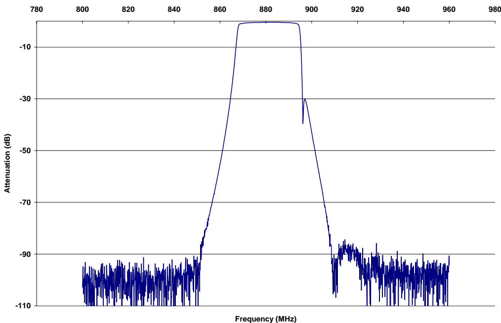
850 RRH 25MHz TX DX Filter
