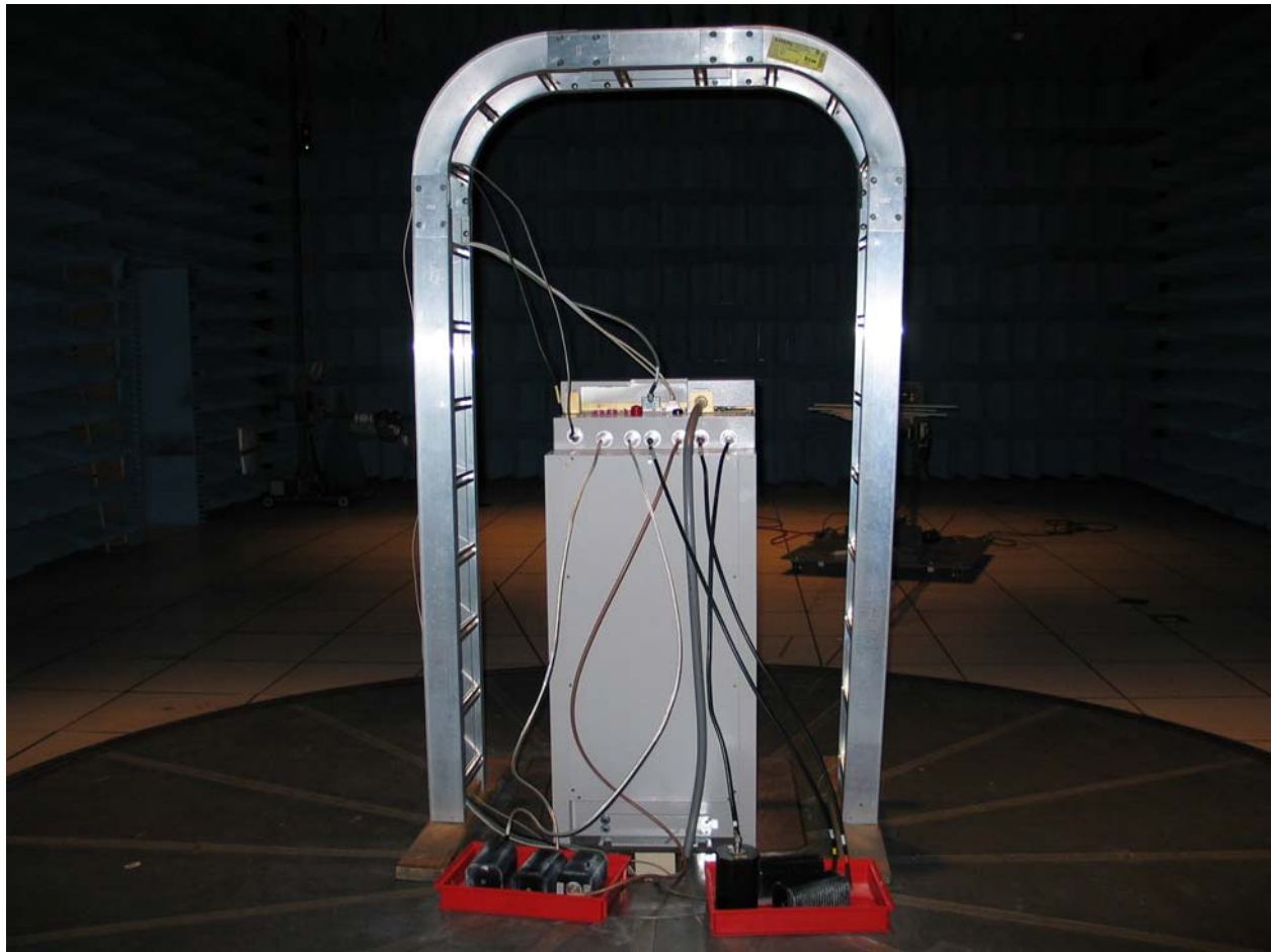
Alcatel-Lucent UMTS CDMA 850 Indoor Base Transceiver Station (BTS) Rear View
