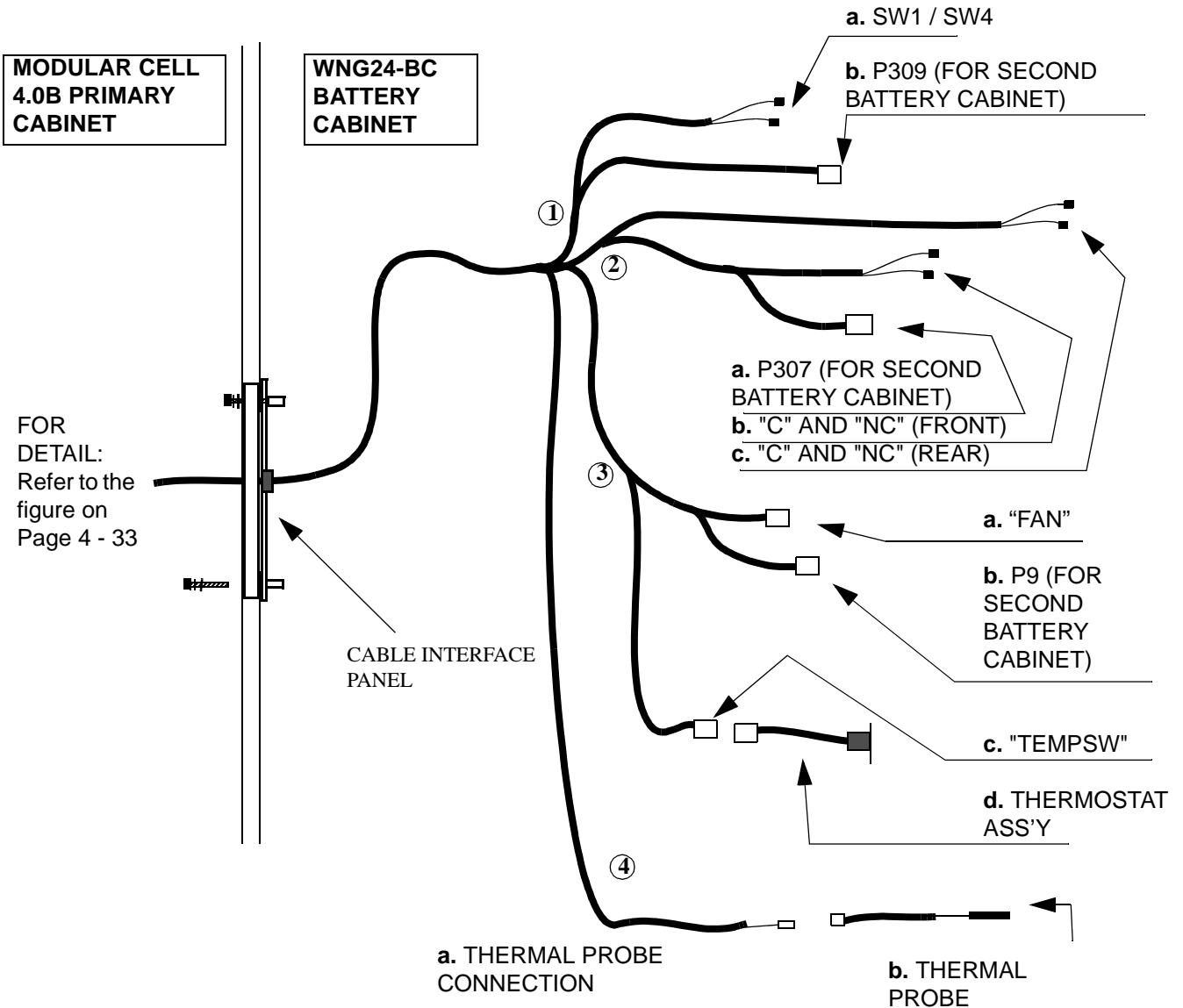
SIDE VIEW FROM FRONT: DC CABLES NOT SHOWN FOR CLARITY
