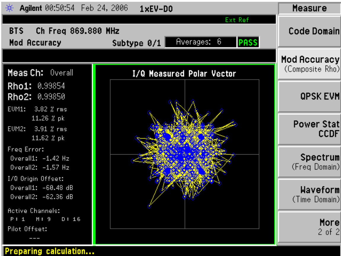
FIGURE 10.3.2 Screen Plot of Mod. Accuracy – IS-856 (3G-1xEV) Overall (pilot, 9 MAC, 16 data)
