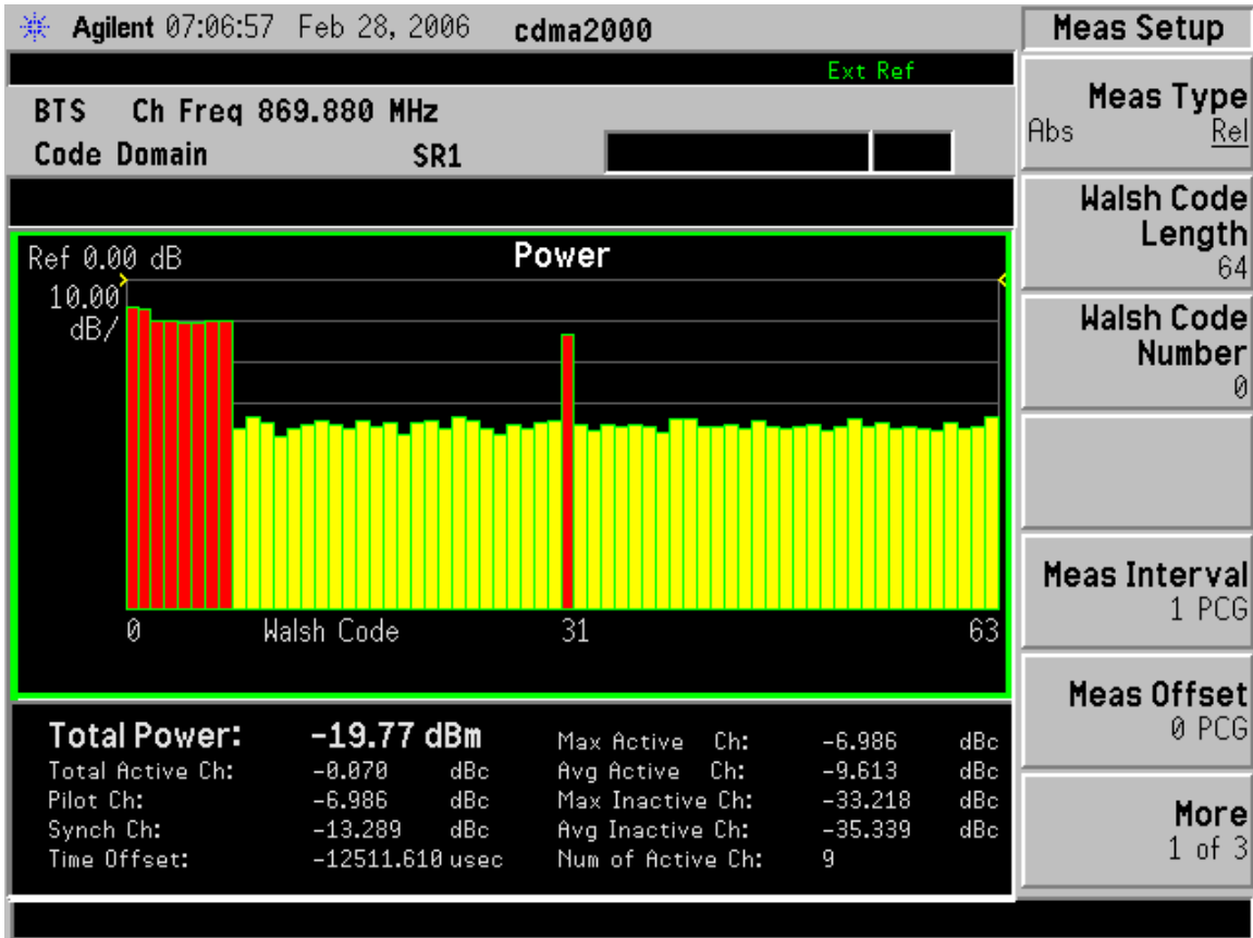
FIGURE 10.3.2 Screen Plot of Code Domain – cdma2000 (3G-1x)
