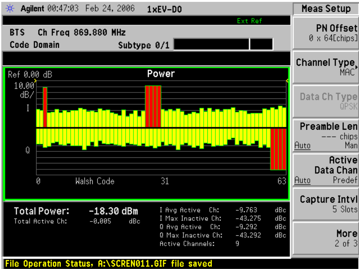
FIGURE 10.3.2 Screen Plot of Code Domain – IS-856 (3G-1xEV) 9 MAC channels
