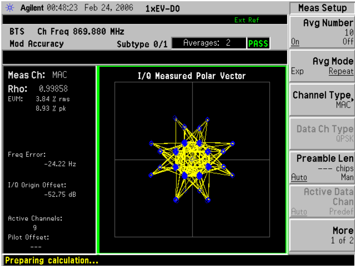
FIGURE 10.3.2 Screen Plot of Modulation Accuracy – IS-856 (3G-1xEV) 9 MAC channels
