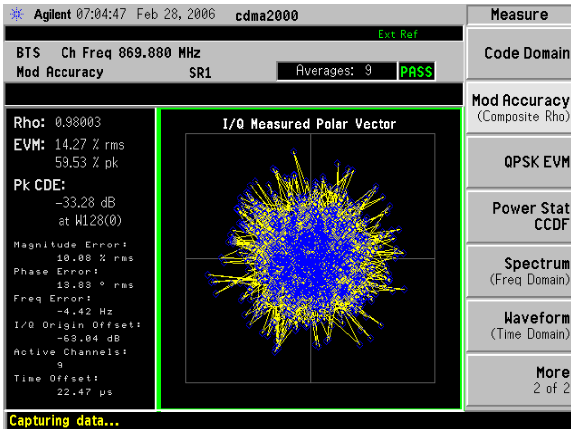
FIGURE 10.3.2 Screen Plot of Modulation Accuracy – cdma2000 (3G-1x)
