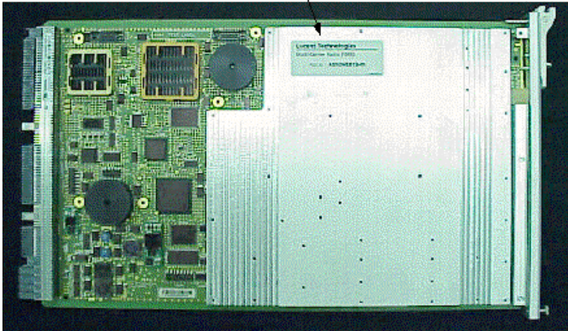
Multi-Carrier CDMA Radio (MCR850), BNJ65
