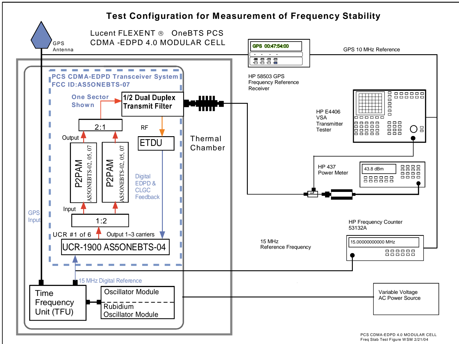
Figure 17 Test Figure for Frequency Stability
