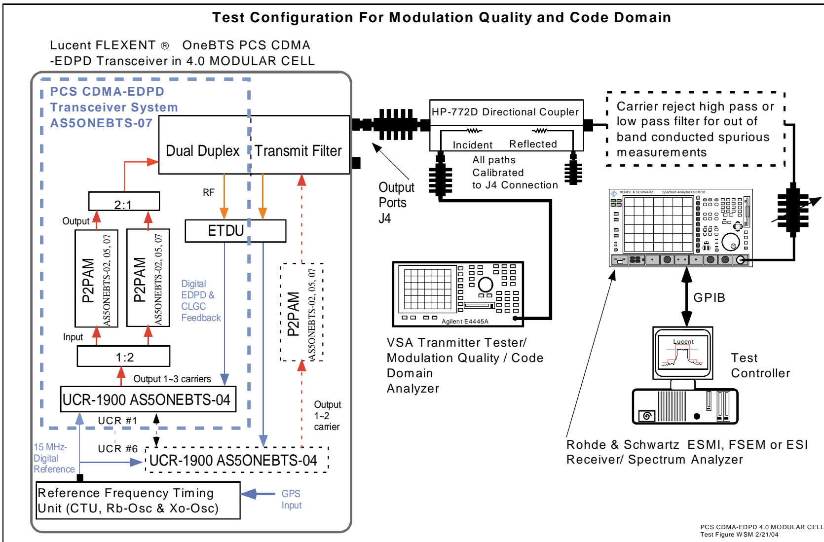
Figure 13 Modulation Quality Measurement
