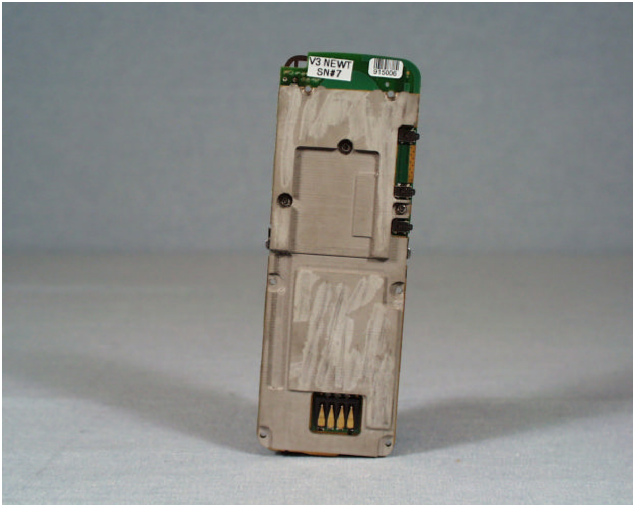
Photograph Showing the Alternate side of PCB with metal weight
