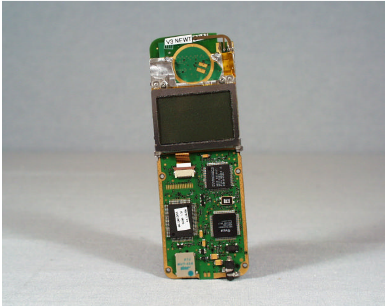
Photograph Showing the Main PCB with LED display
