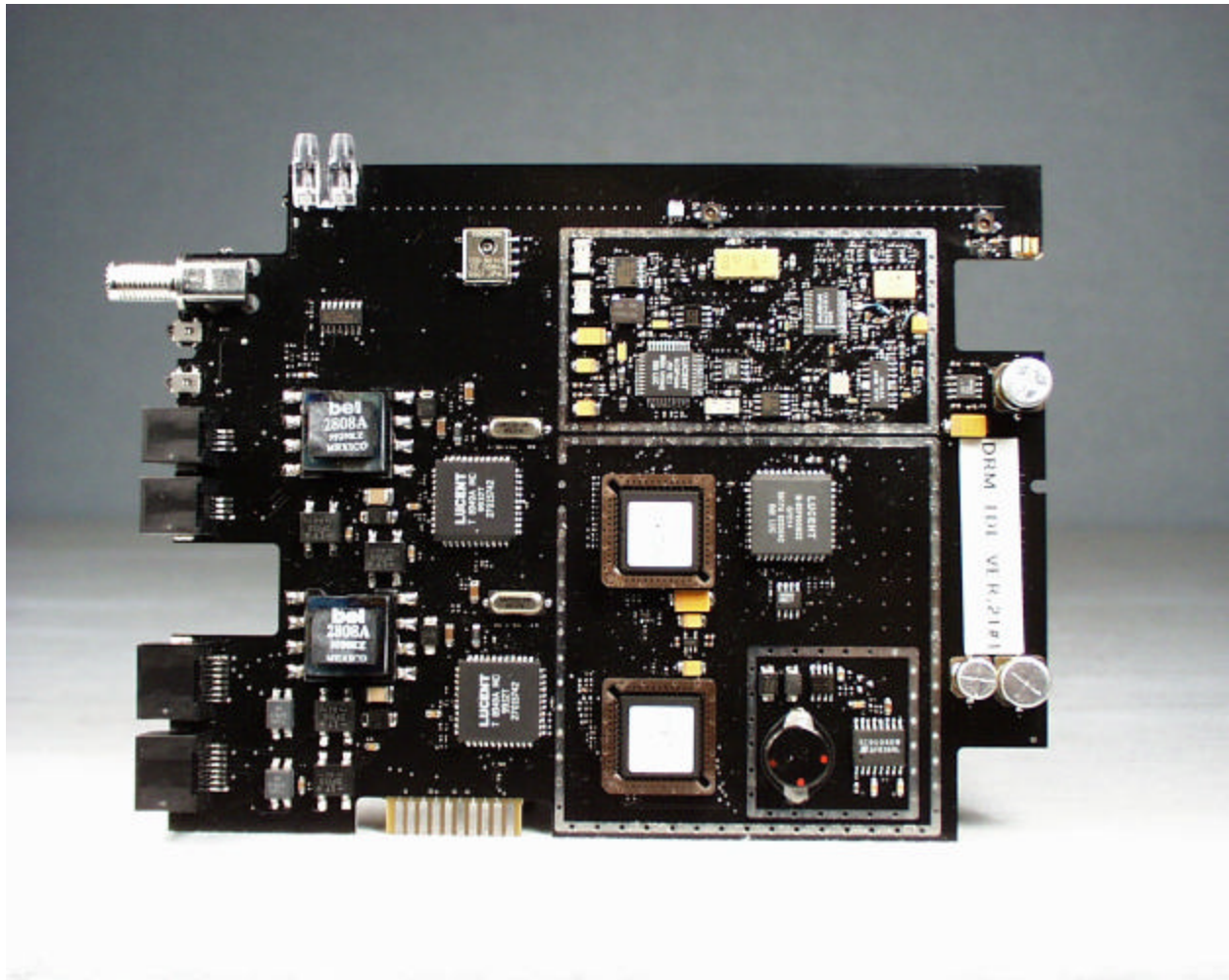
Component Side of DCM PCB without Shields Installed (Base)
