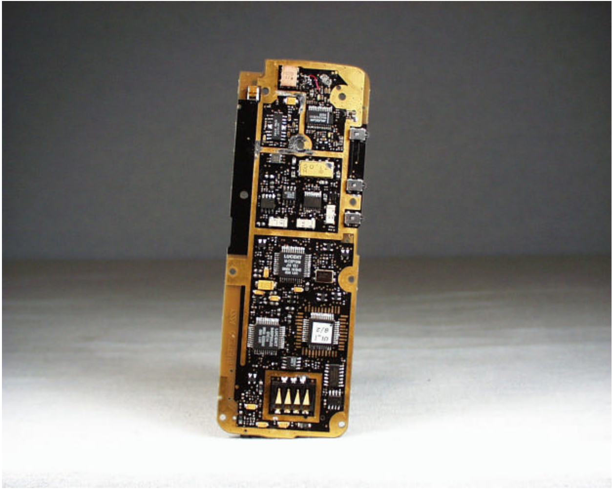
Opposite Side of PCB without Shield Installed (Handset)
