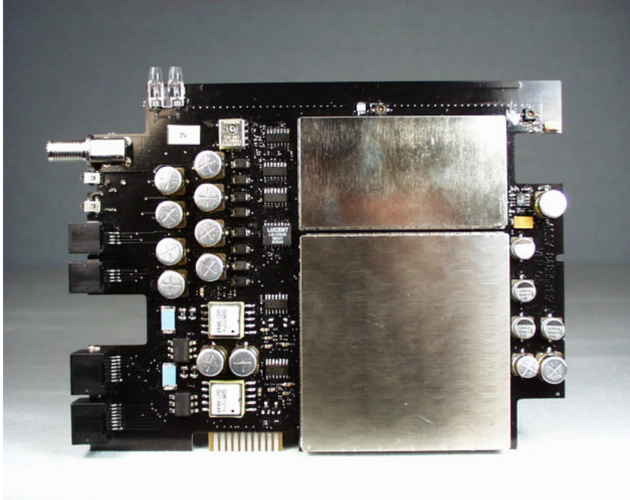
Component Side of ETR with Shields Installed PCB (Base)
