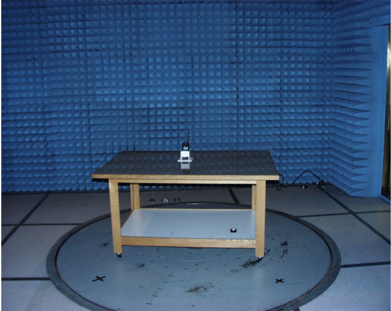
Front view of worst case radiated emissions (Handset)
