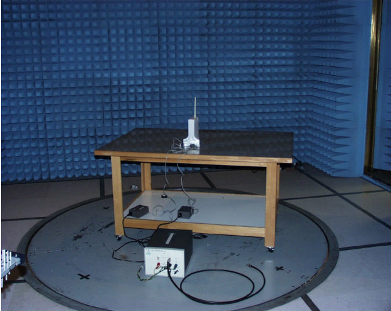
Back view of worst case radiated emissions (Base)
