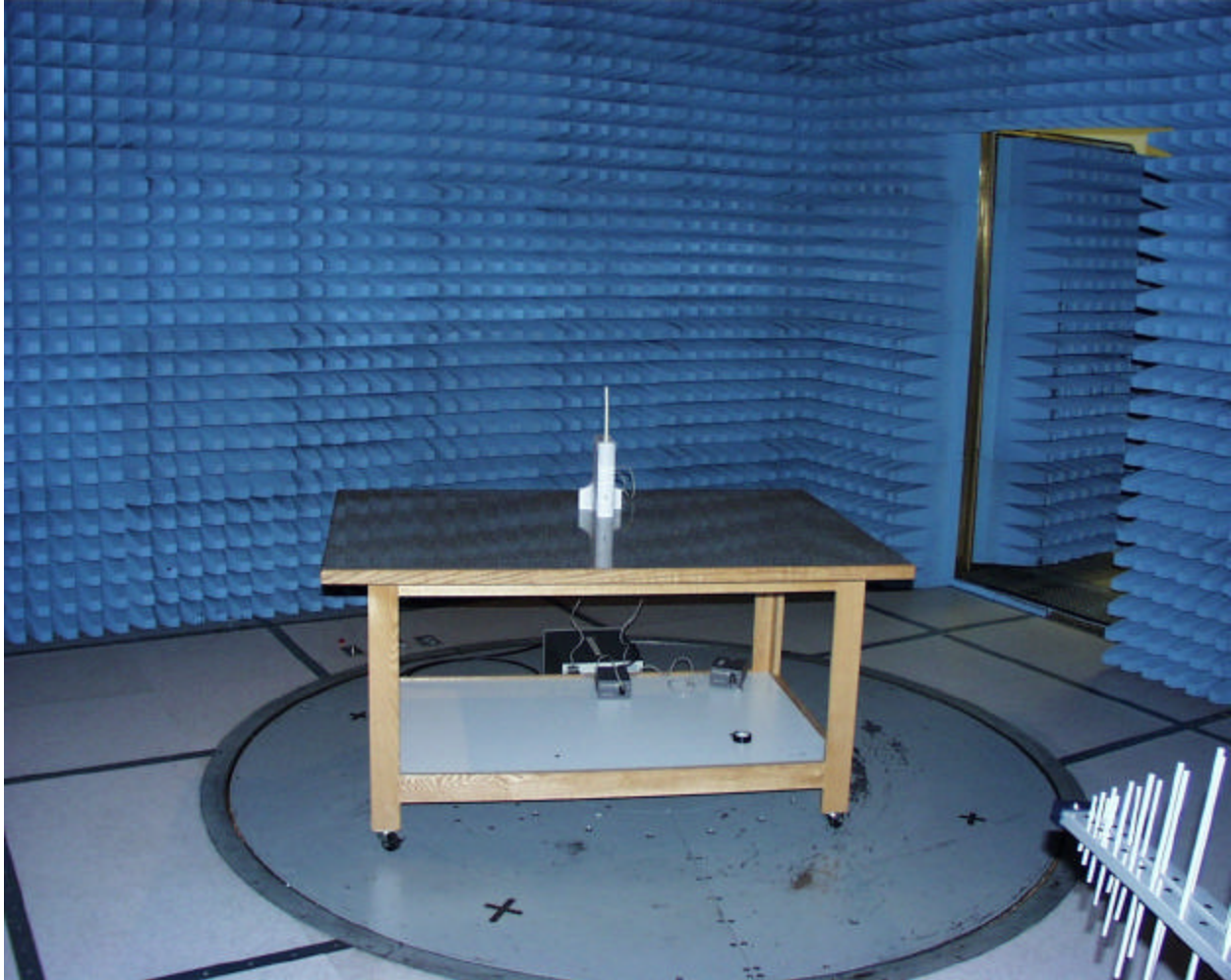
Front view of worst case radiated emissions (Base)
