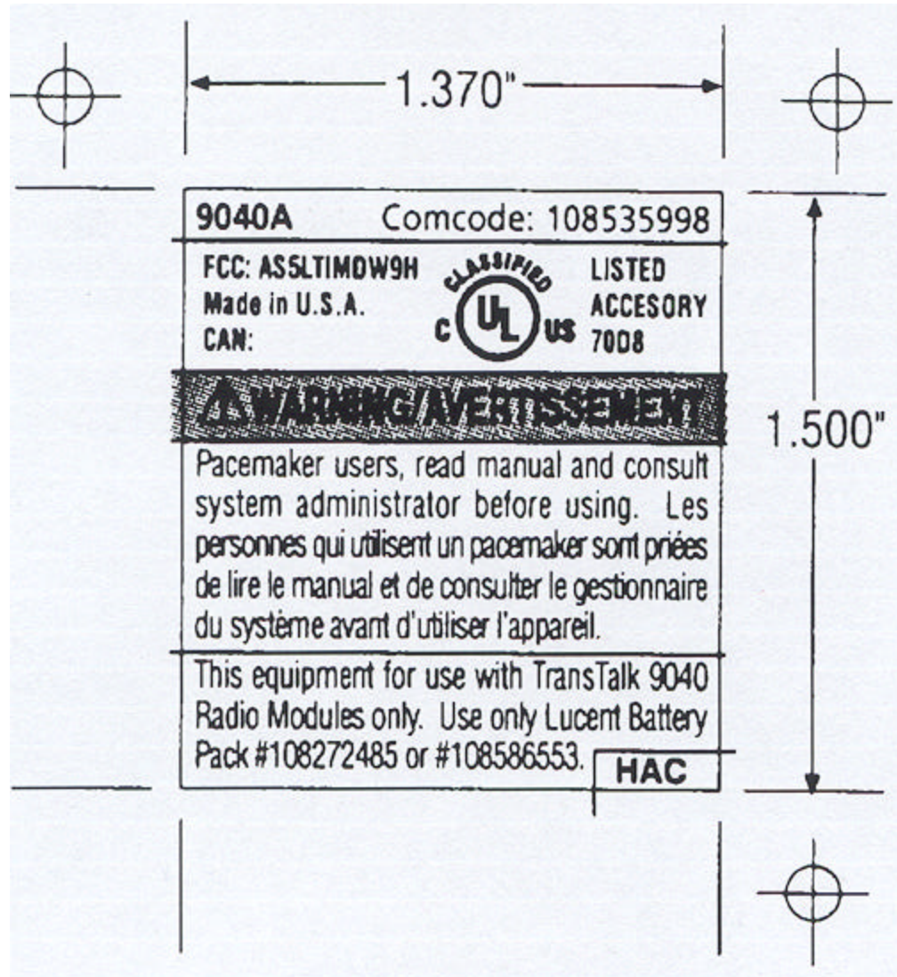
Sketch of the label on the back exterior of the handset.
