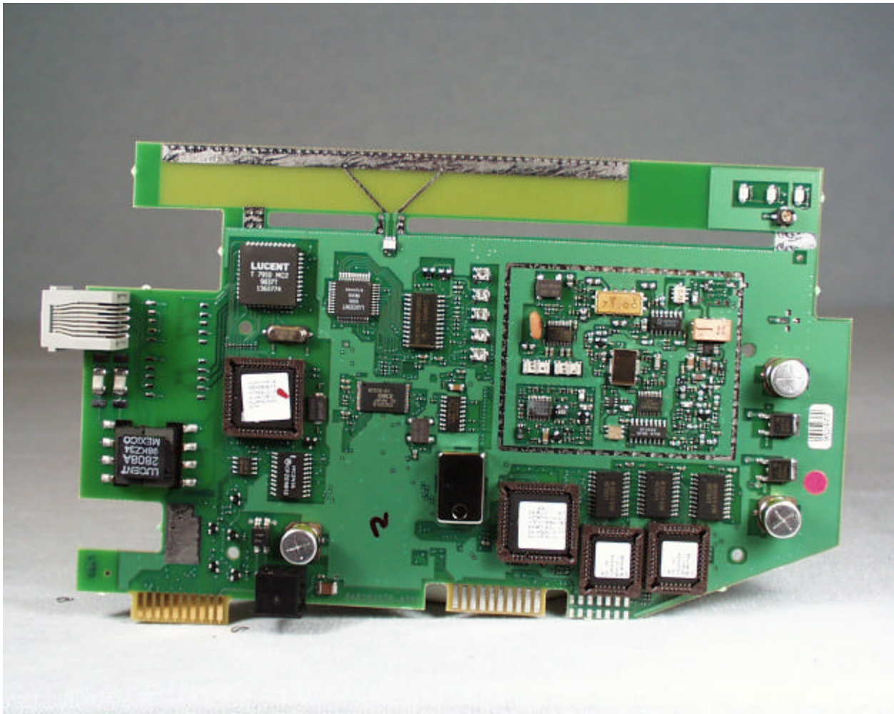
Opposite Side of PCB with RF cans removed (Base)
