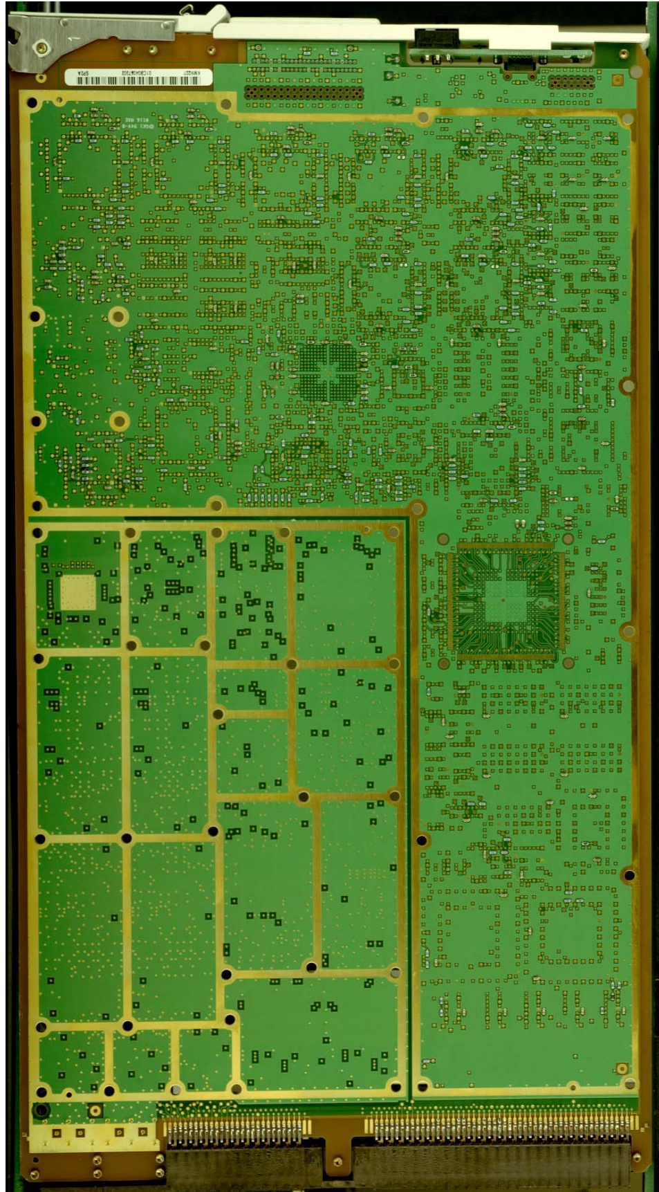
AS5CMP-40 SBEDRU Transceiver Circuit Board Wiring Side View With Shielding Cover Removed
