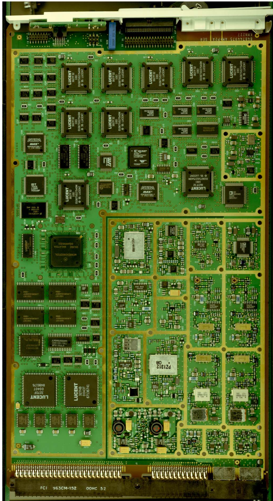
AS5CMP-40 SBEDRU Transceiver Circuit Board Component Side View With Shielding Cover Removed
