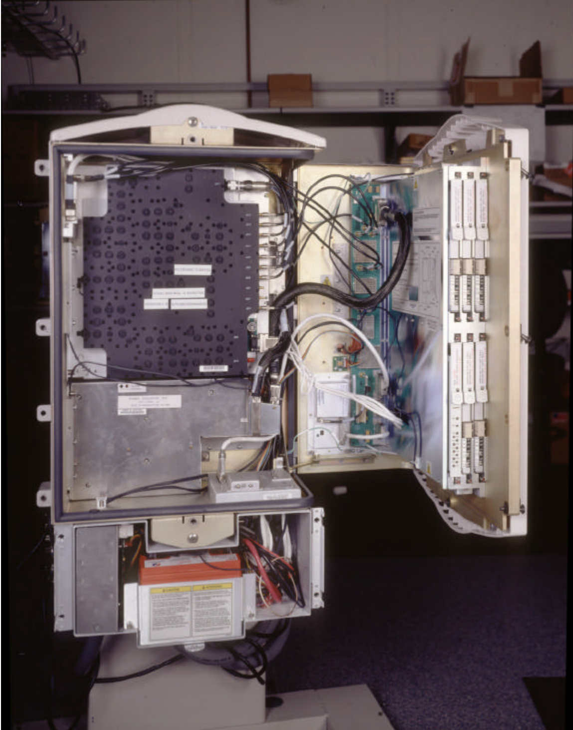
FLEXENT™ Cellular TDMA Microcell J41698B-1: Interior View
