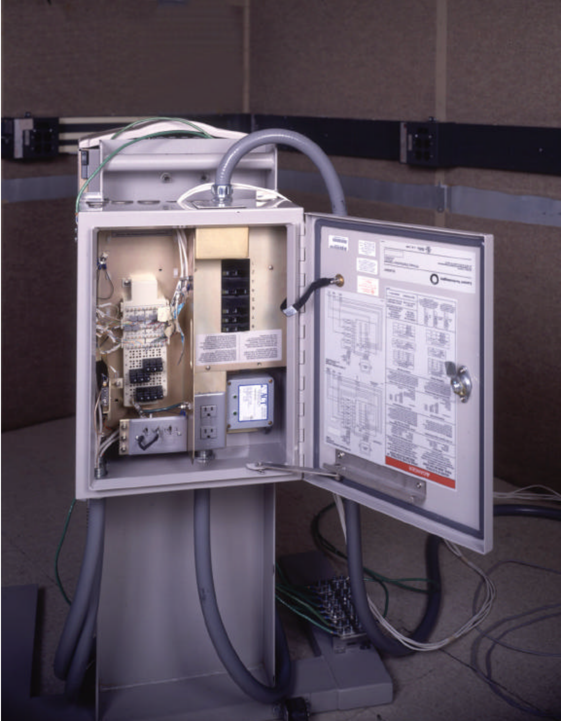
FLEXENT™ Cellular TDMA Microcell J41698B-1: Primary Distribution Cabinet Interior View
