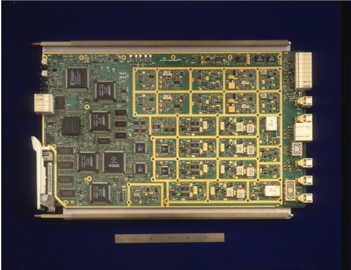
Cellular TDMA Dual Radio Module 44WR54: Circuit Board View
