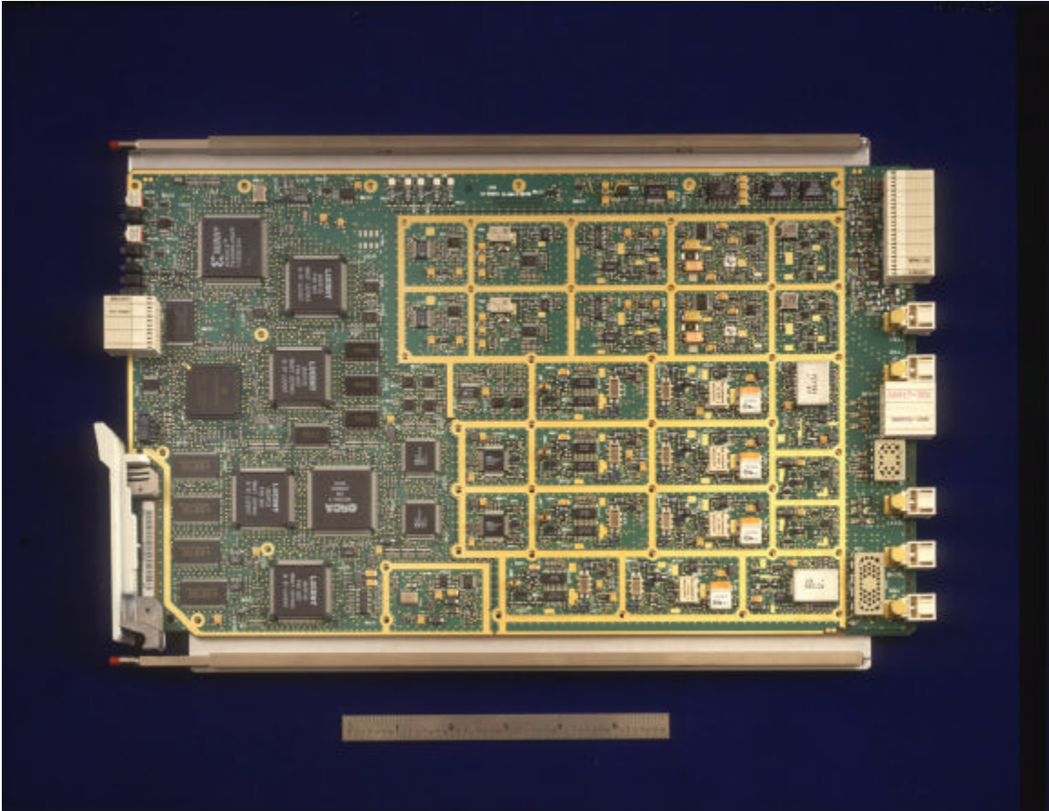
PCS-TDMA Dual Radio Module 44WR53: Circuit Board View
