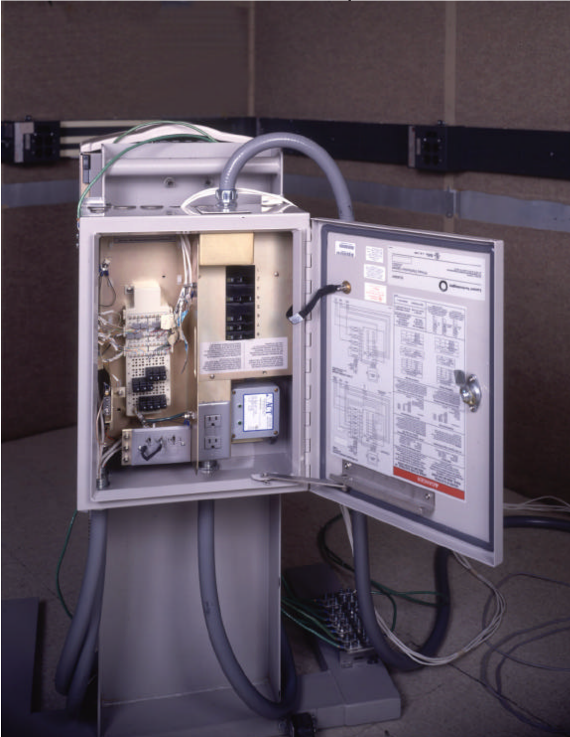
FLEXENT™ PCS-TDMA Microcell J41698A-1: Primary Distribution Cabinet Interior View
