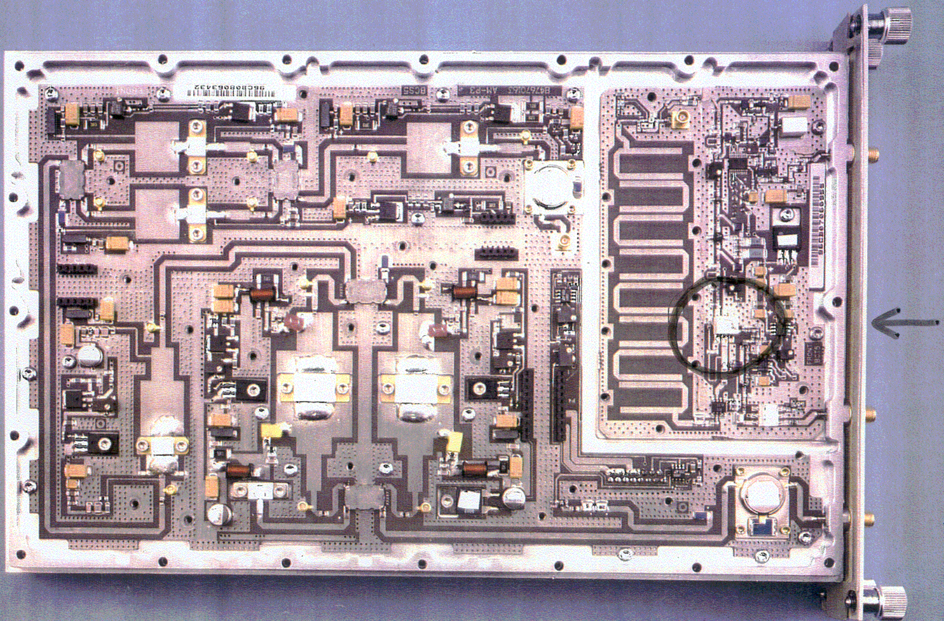
FCC ID: AS5CMP-19 Exhibit 20 PCS-TDMA Transmit Unit 44WA14 Fig 6.: RF Board
