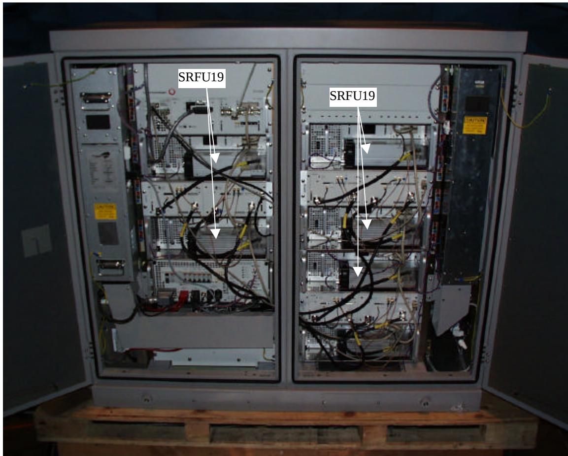
Photo Shows SRFU19 Installed in a BTS2000/60dB Cabinet
